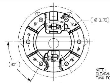
DETAIL A SCALE 1:2 VALVE ORIENTATION SHOWN AS REFERENCE
