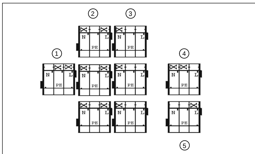
Fig. 9 Rear view of the panel 302 - terminal assignment
