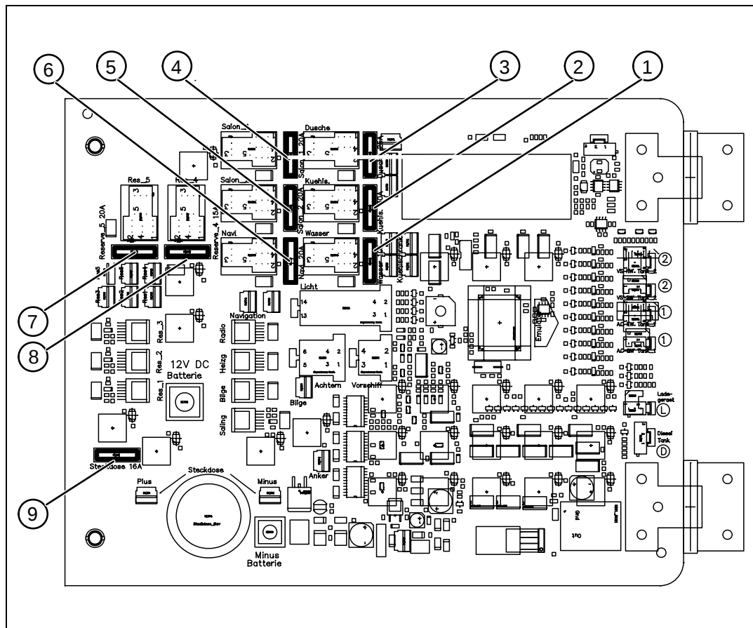
Fig. 8 Rear view of the panel 301 - micro-fuses
