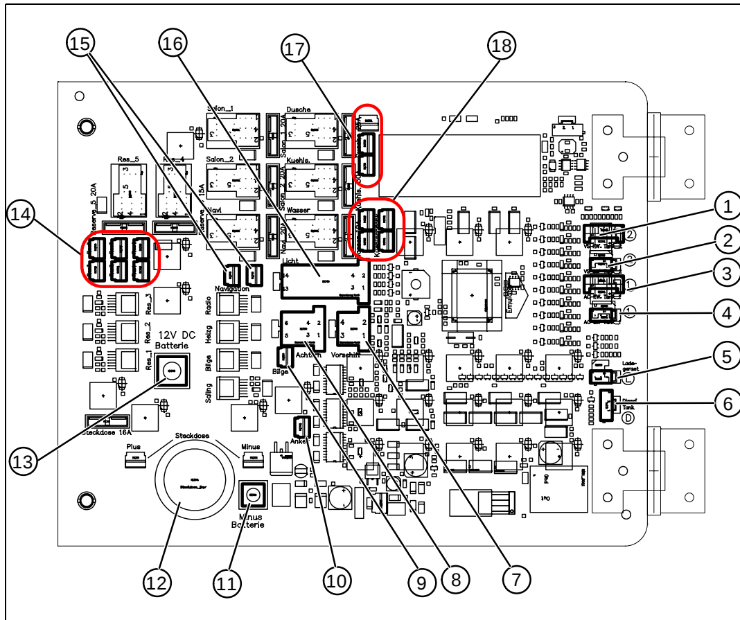
Fig. 7 Rear view of the panel 301 - terminal assignment
