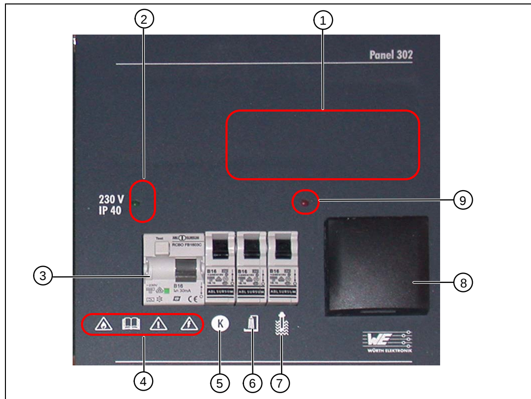
Fig. 6 Overview of panel 302
