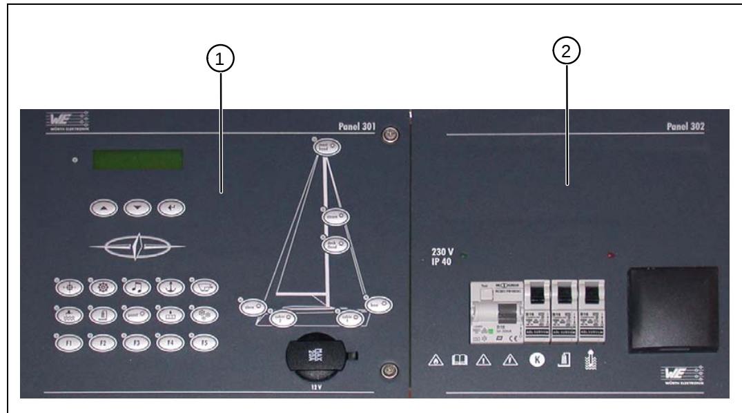
Fig. 1 Overview - panel 301/302
