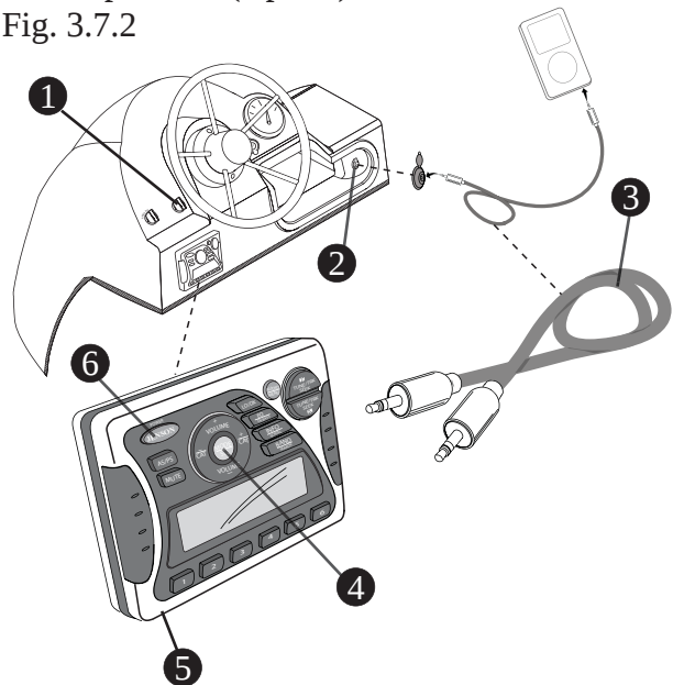
MP3 Operation (Option)
