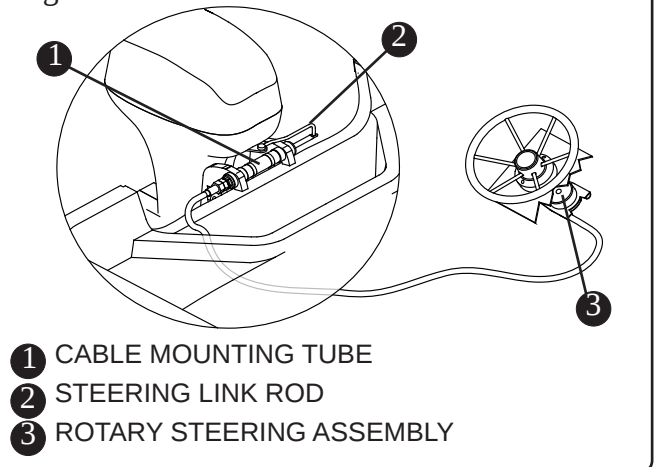
No-Feedback Steering (Typical) Fig. 2.13.2
