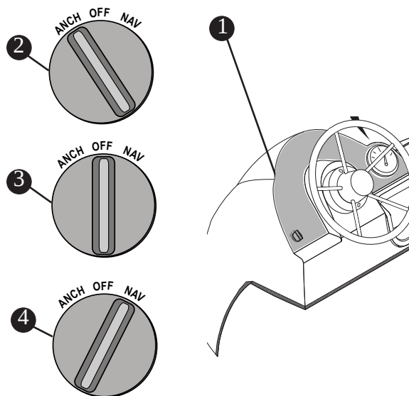
NAV/ANCH Switch Positions Fig. 2.12.2
