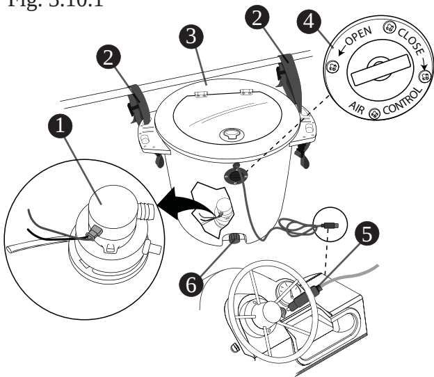
Carry-On Livewell (Option) Fig. 3.10.1
