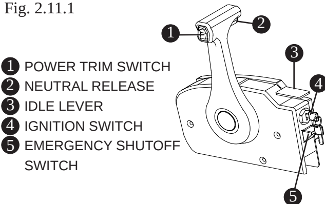
Gear shift/Throttle Fig. 2.11.1
