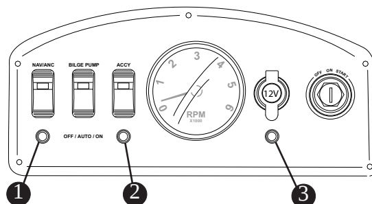
Component Circuit Breakers Fig. 4.2.2
