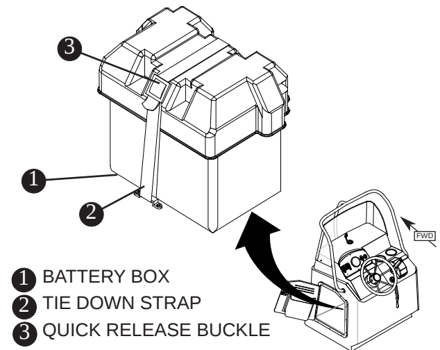
Battery Box Fig.4.1.1
