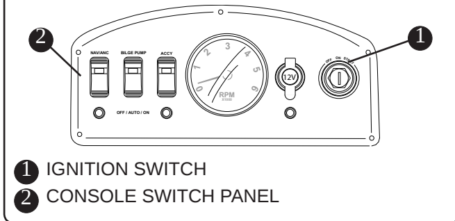
Ignition Switch Fig. 3.6.1
