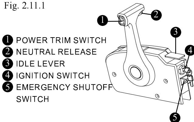
Gear shift/Throttle
