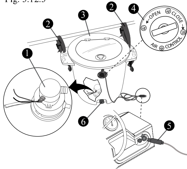
Carry-On Livewell (Option) Fig. 3.12.3
