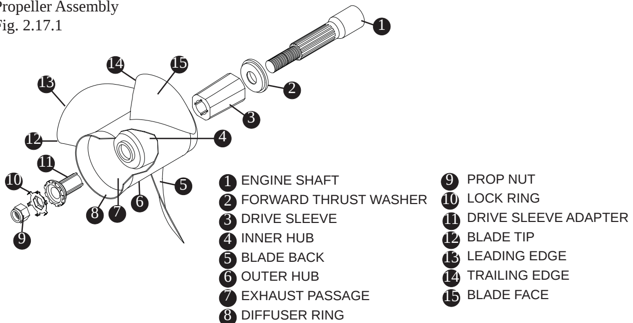
Propeller Assembly
