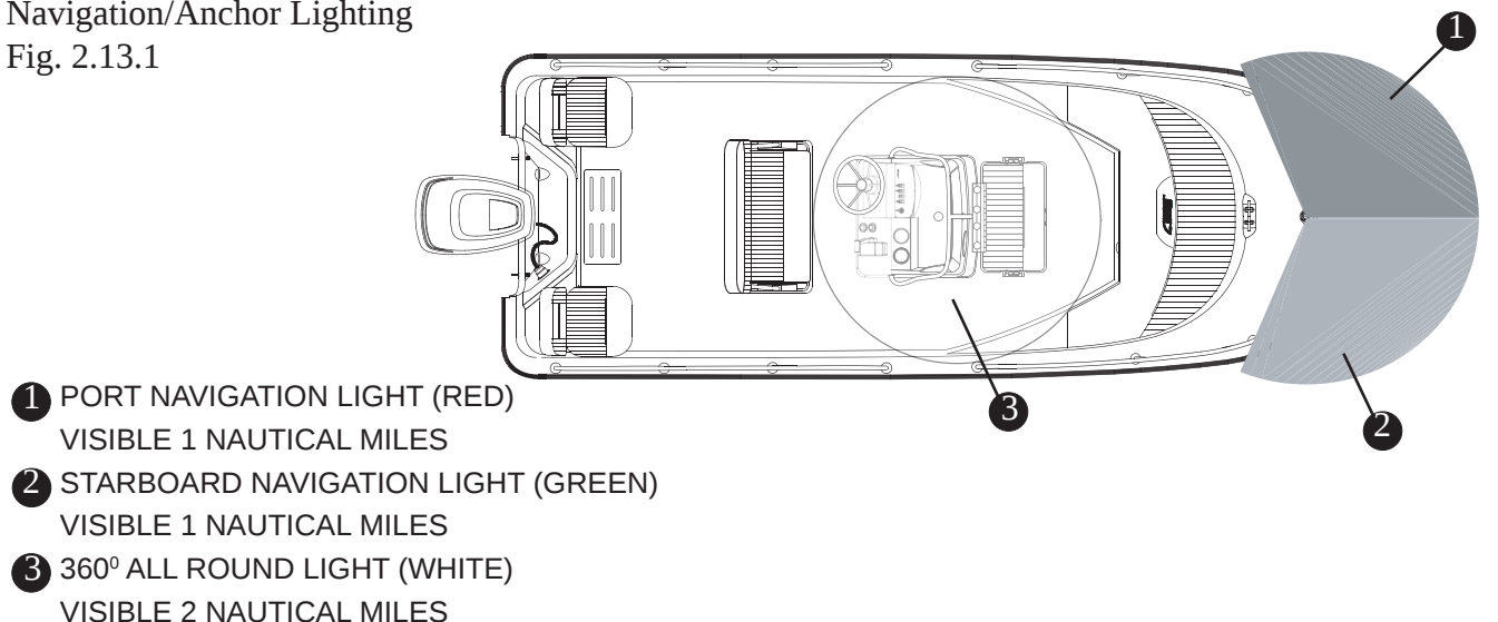
Navigation/Anchor Lighting
