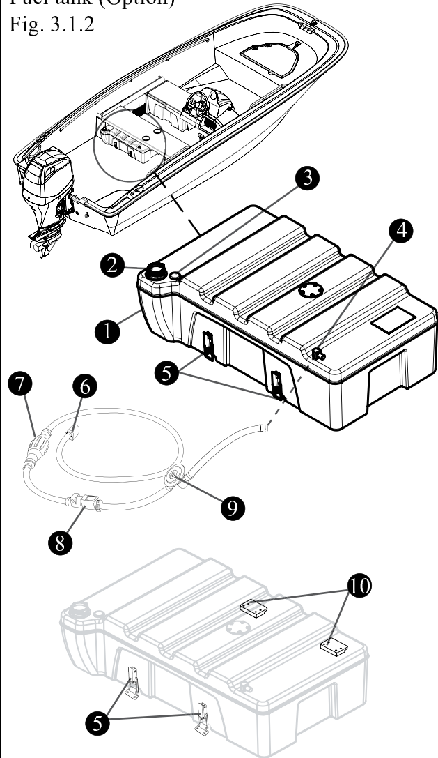
Fuel tank (Option)
