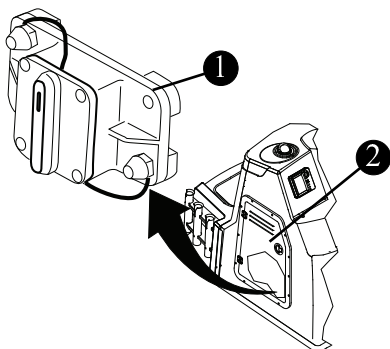
Trolling Motor Receptacle Breaker (Option) Fig. 4.3.1
