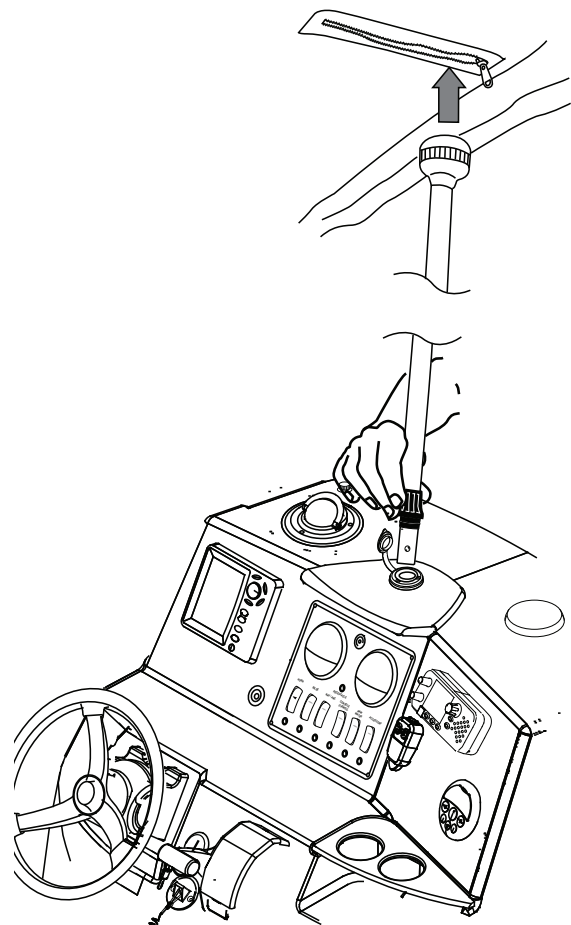
Anchor Light Installation Fig. 2.15.1
