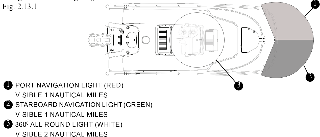
Navigation/Anchor Lighting
