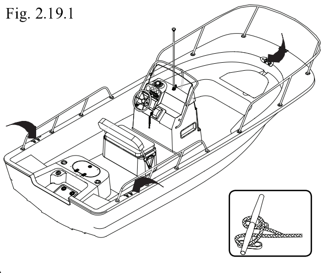
Cleat Locations
