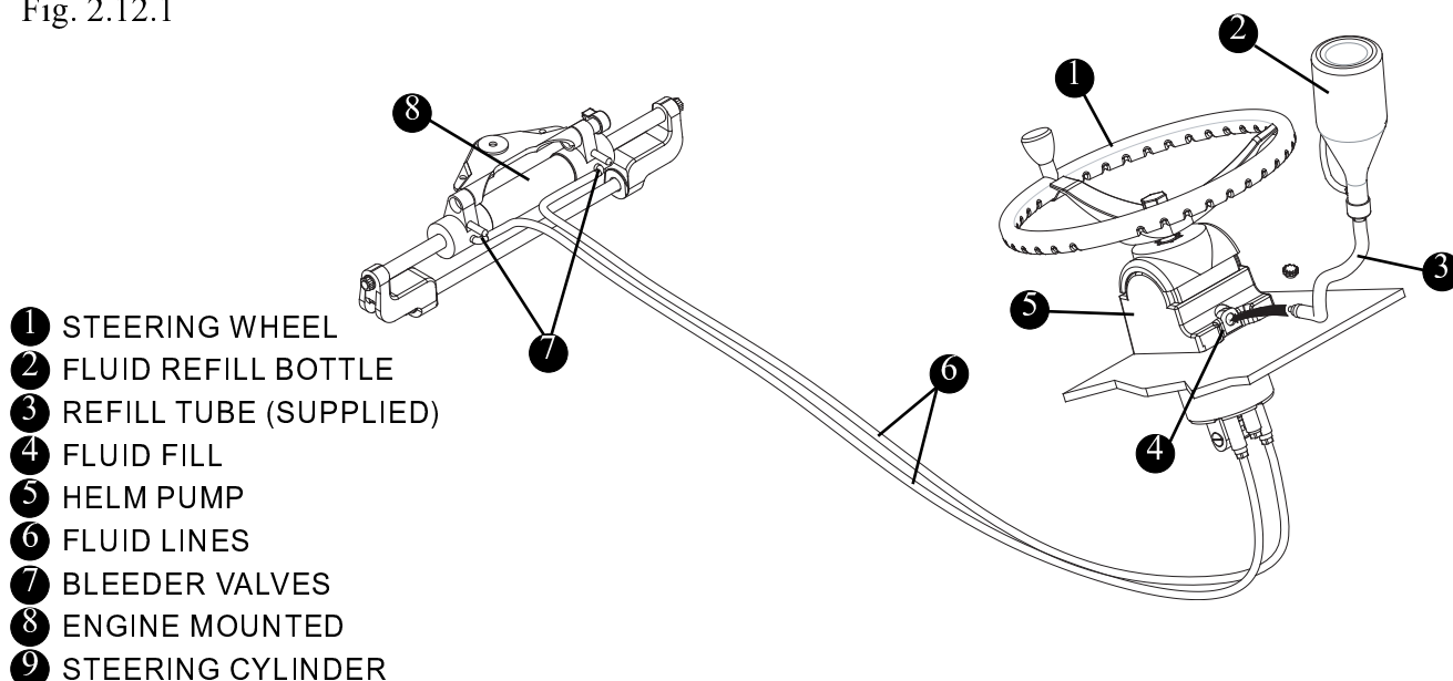
Hydraulic Steering Fig. 2.12.1
