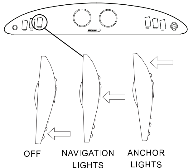
Navigation/Anchor Lighting Switch Fig. 2.15.2
