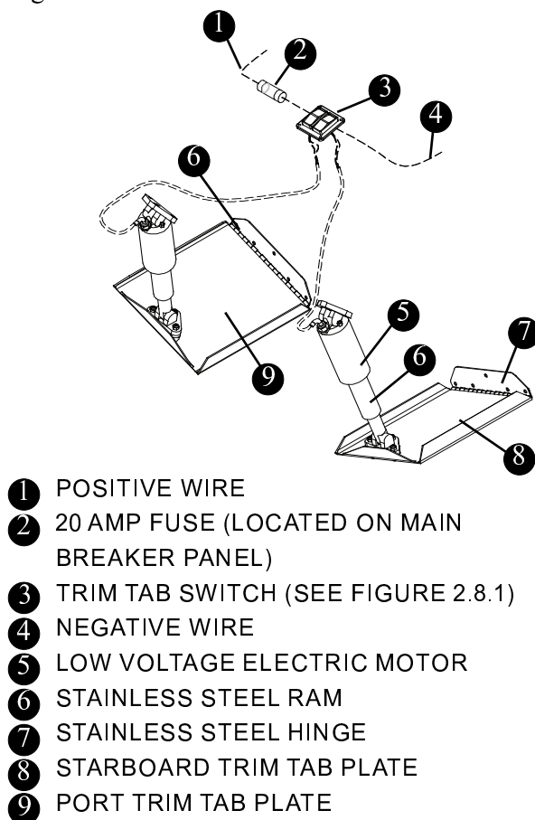
Electrically Powered Trim Tabs (Optional) Fig. 2.16.1
