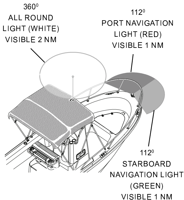
Navigation/Anchor Lighting Fig. 2.15.1
