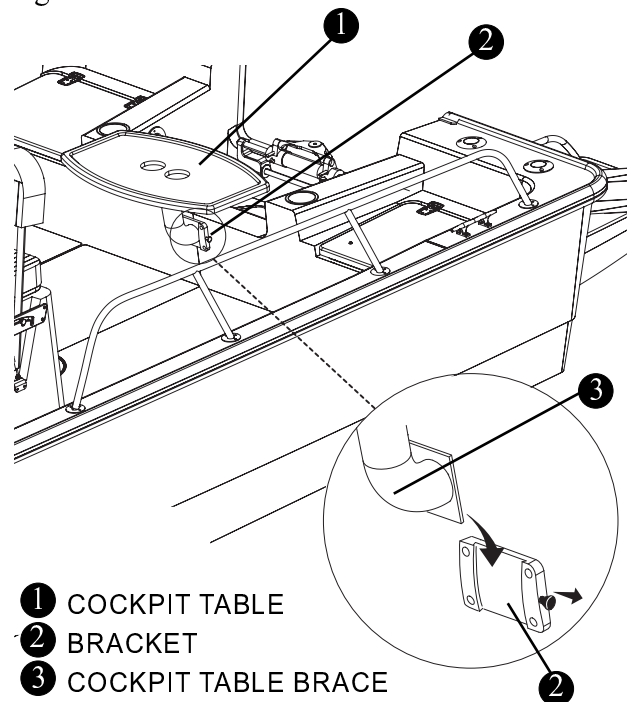
Cockpit Table Installation (Option) Fig. 3.14.2
