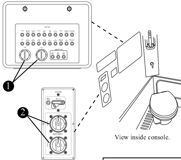
Battery Switch Panel Fig. 3.8.1
