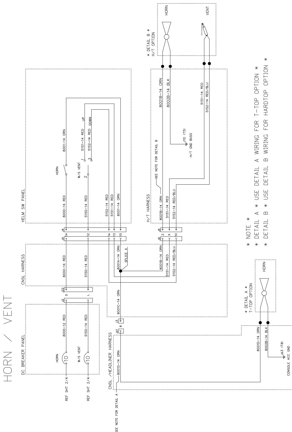
250 Outrage Schematic - Sheet 14 Fig. 4.22.1
