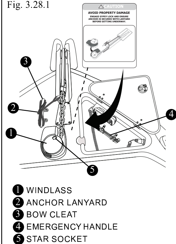
Windlass Manual/Emergency Operation Fig. 3.28.1
