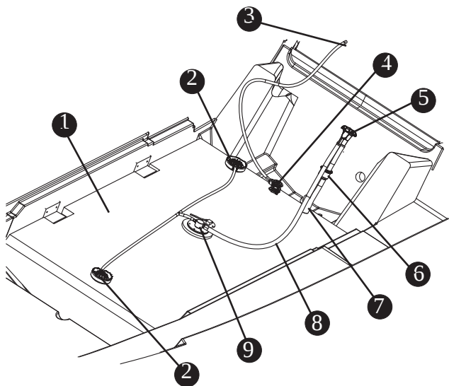
Fuel Tank Fig. 3.3.1
