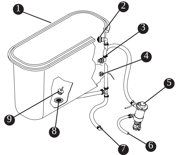
Reversible Pilot Seat w/Livewell (Option) Fig. 3.9.2
