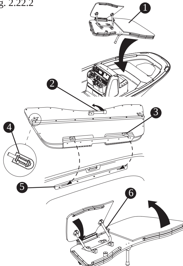
Adjustable Sun Lounge (Option) Fig. 2.22.2
