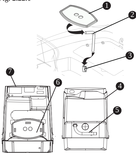
Bow Table Installation & Storage (Option) Fig. 2.22.1
