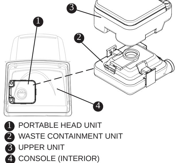
Portable Head Unit Fig. 3.12.1
