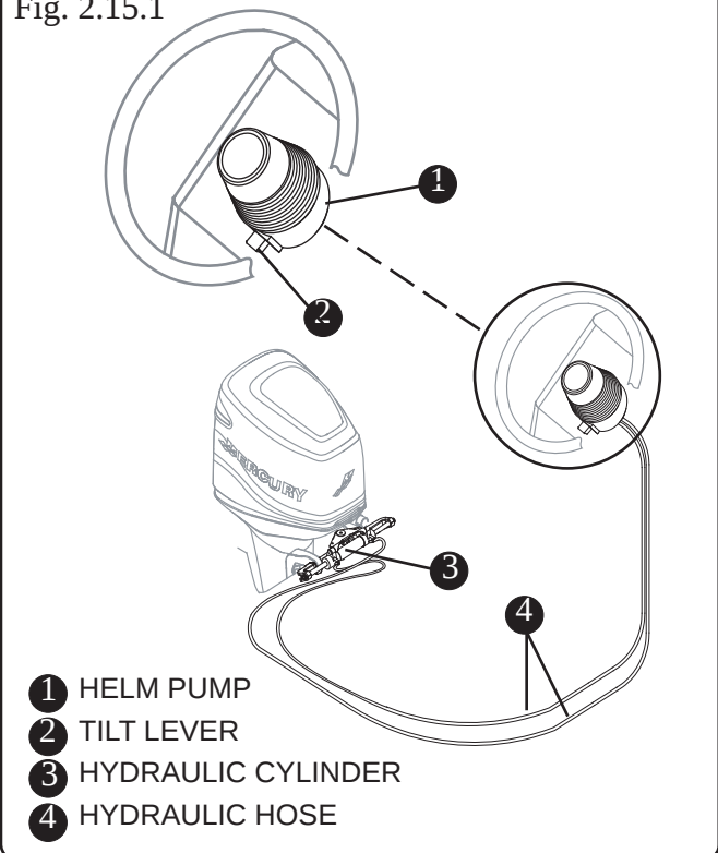
Hydraulic Tilt Steering Fig. 2.15.1
