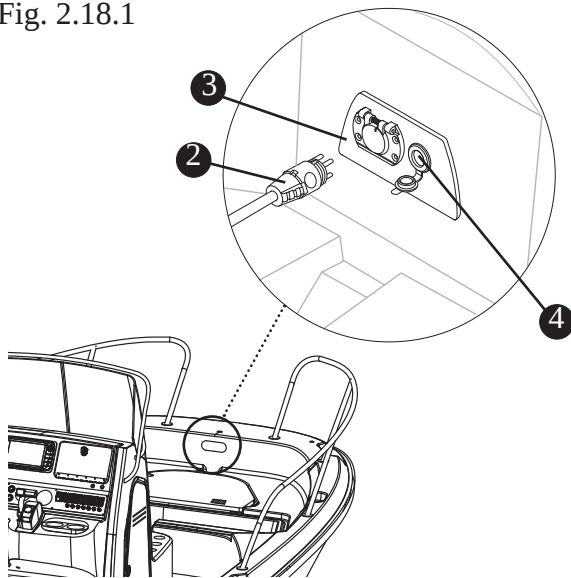
Trolling Motor Panel (Option)
