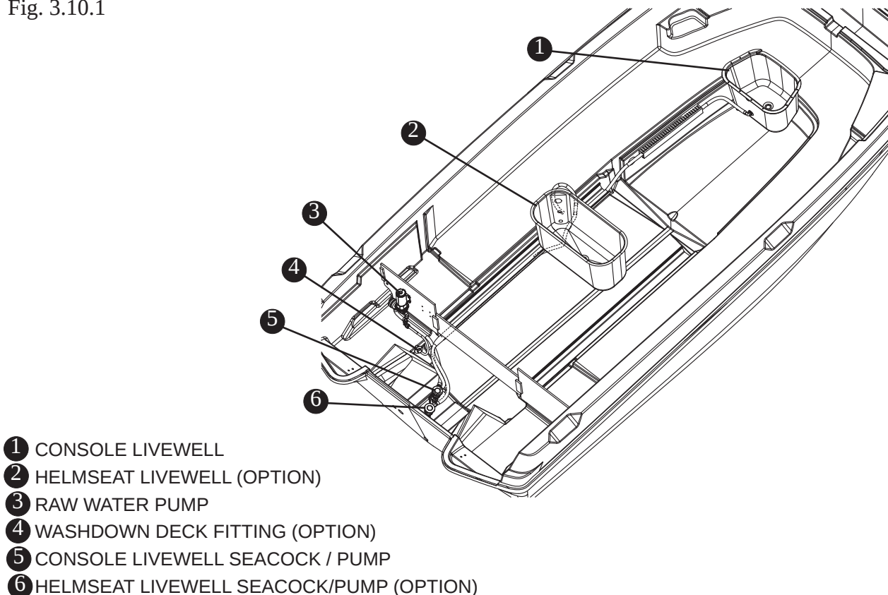
Raw Water System Fig. 3.10.1
