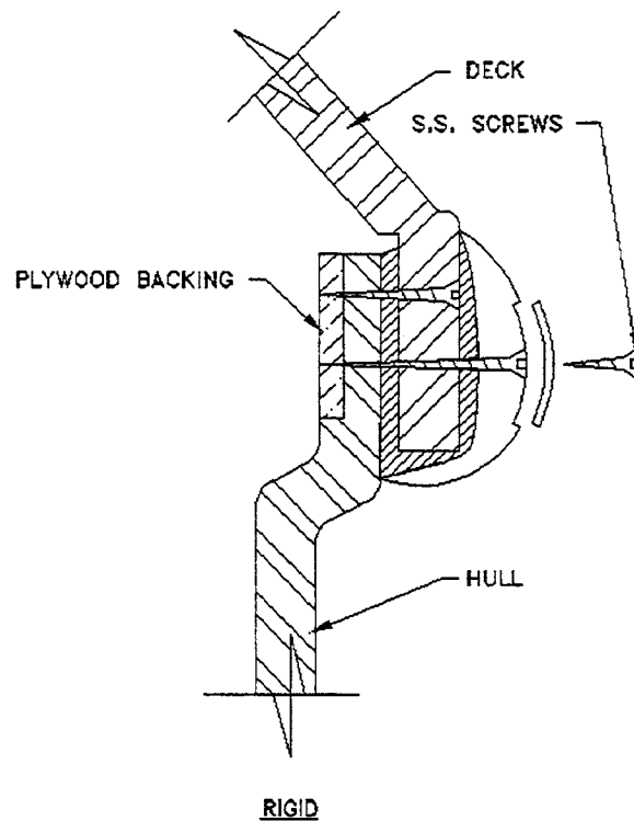
Carver "shoe box" hull-to-deck joint
