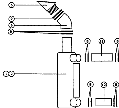
TYPICAL MUFFLER INSTALLATION (PORT SHOWN)
