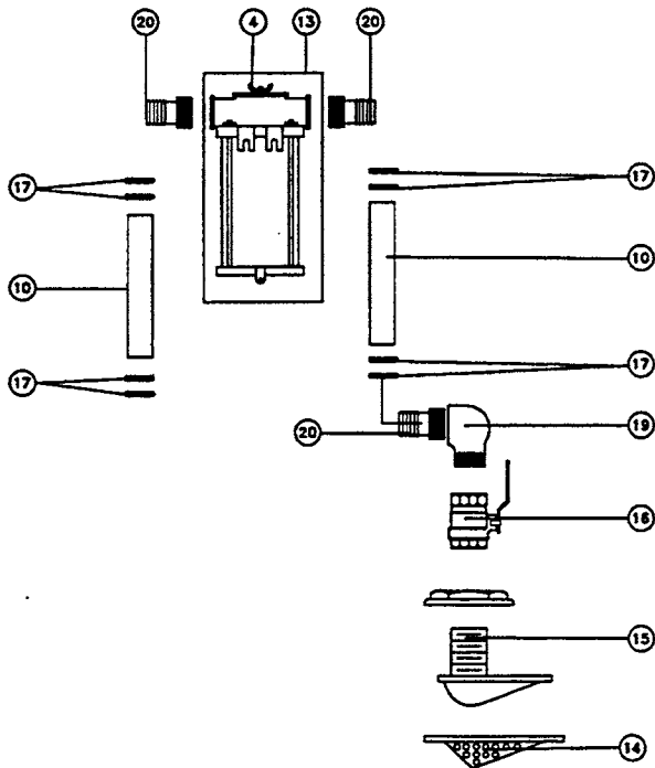
TYPICAL INTAKE INSTALLATION
