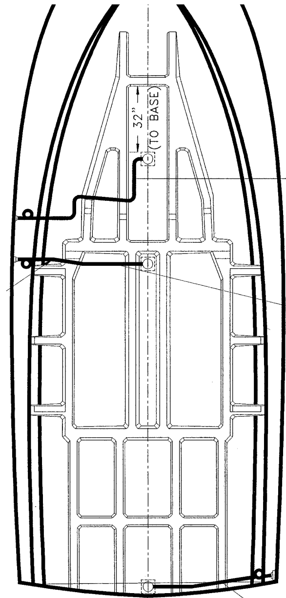
BILGE SYSTEM
