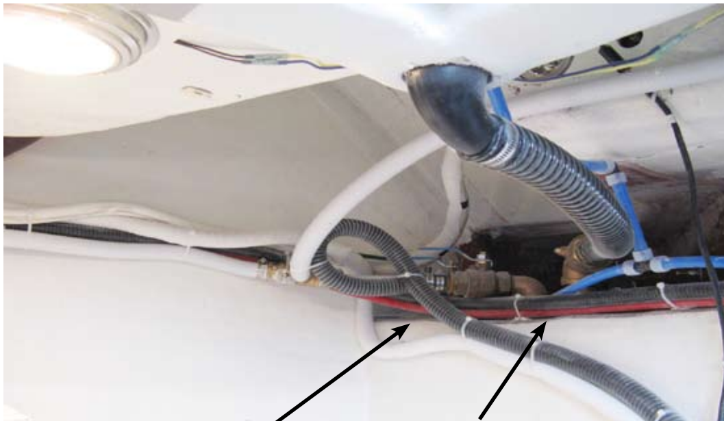
Drains for aft transom area (starboard) shown in open position.
