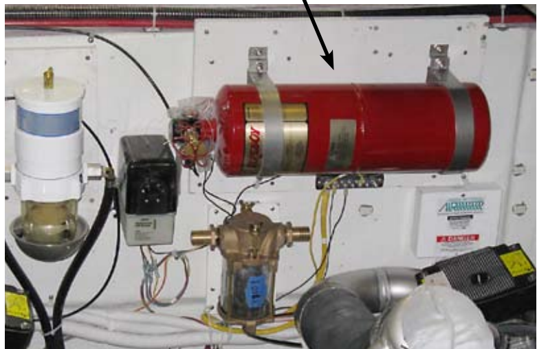
Fire Suppression Tank (Transom Port Side)
