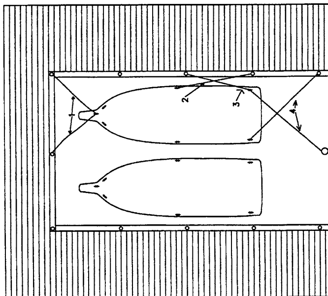
Mooring Illustration
