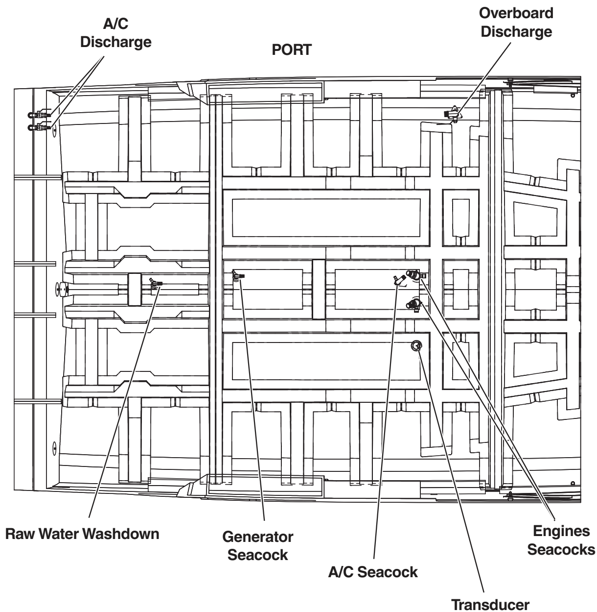
Figure 9-3 – Aft Thru-hull Valves
