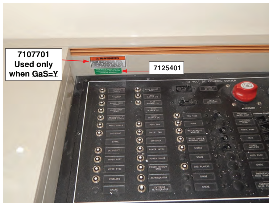
Figure 2-7 – Labels Required at 12V Panel
