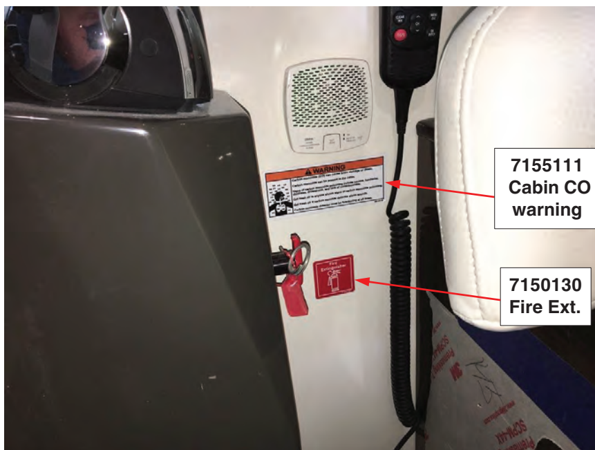
Figure 2-4 – CO and Fire Extinguisher Labels Place din Salon Area
