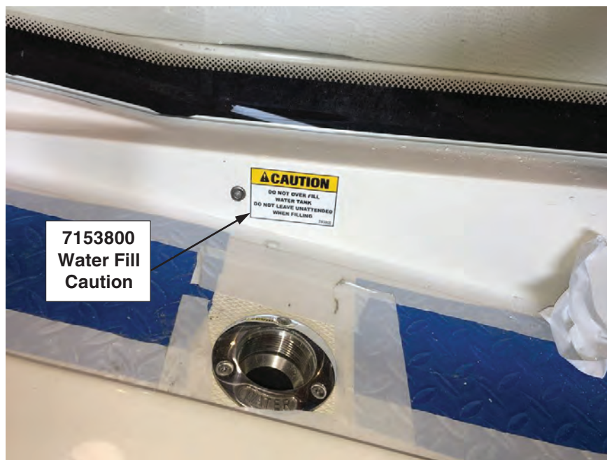
Figure 2-11 – Caution Label at Water Fill Deck Plate
