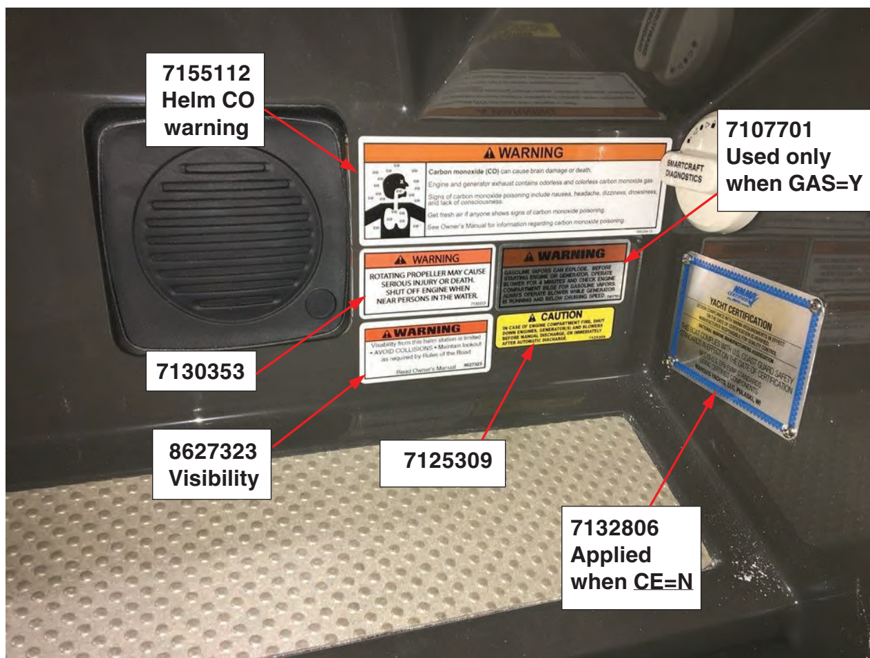
Figure 2-1 – Label Placement at Helm
