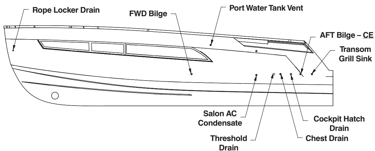
Figure 9-2 – Port Thru-Hull
