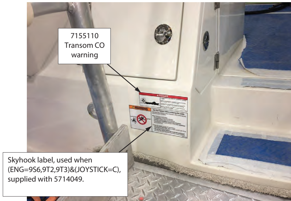
Figure 2-10 – Labels Placed on Transom
