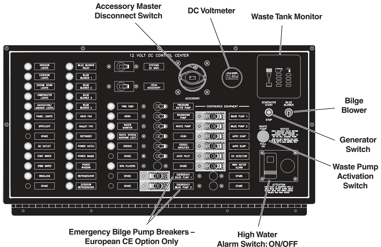
Figure 7-7 – DC Control Center
