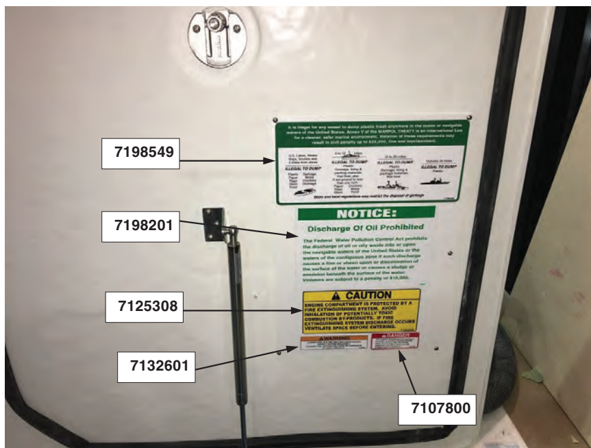
Figure 2-8 – Labels Placed on Underside of Engine Room Hatch
