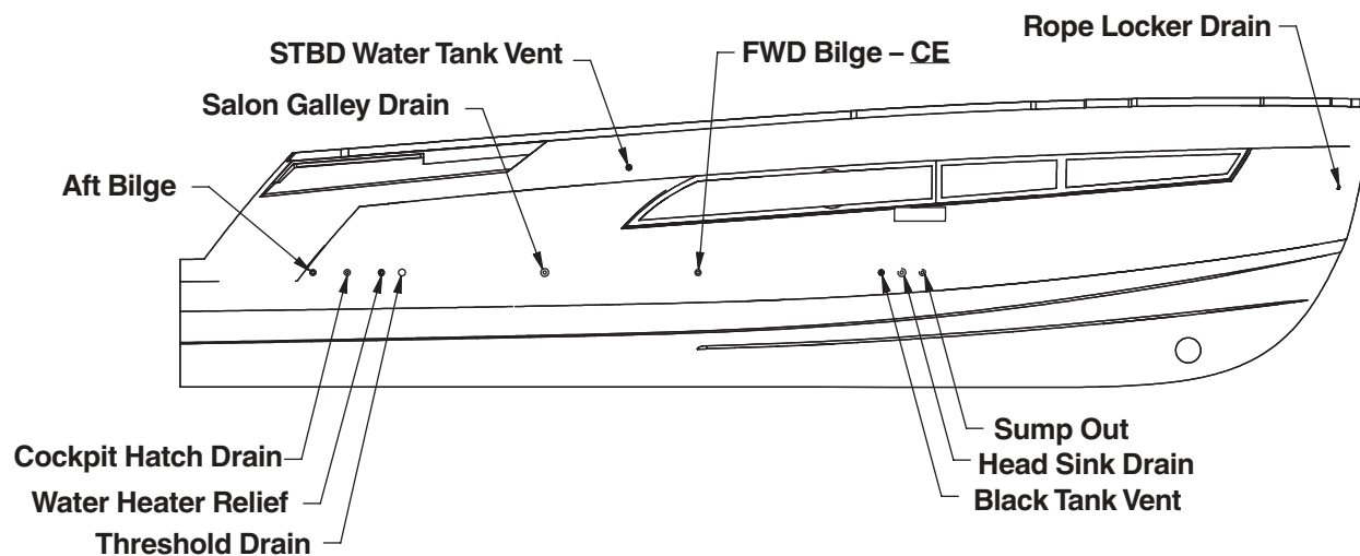
Figure 9-1 – Starboard Thru-Hull
