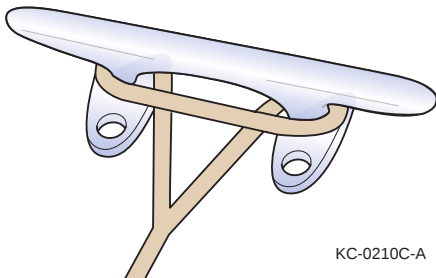
Figure 8-9 – Cleating an Eye Spliced Line
