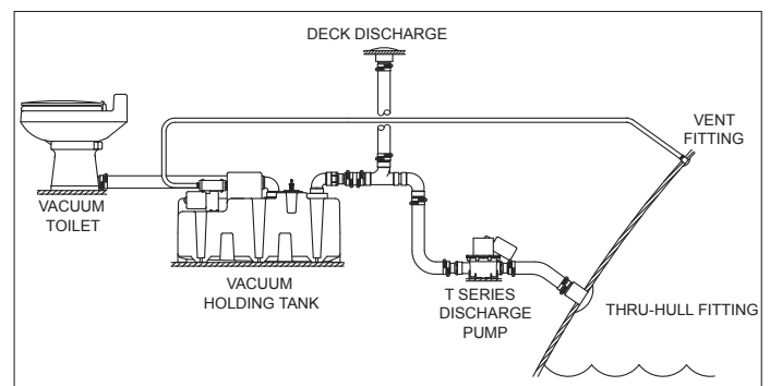
Figure 3.3 VacuFlush® Head
