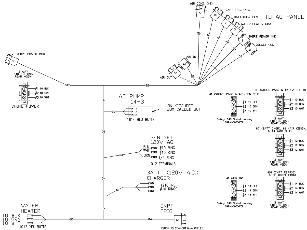
AFT AC HARNESS
