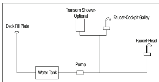
Optional Pressure Water System
