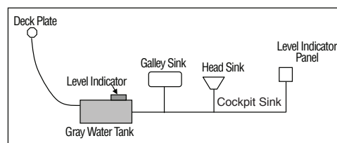
Figure 3.4 Gray water System
