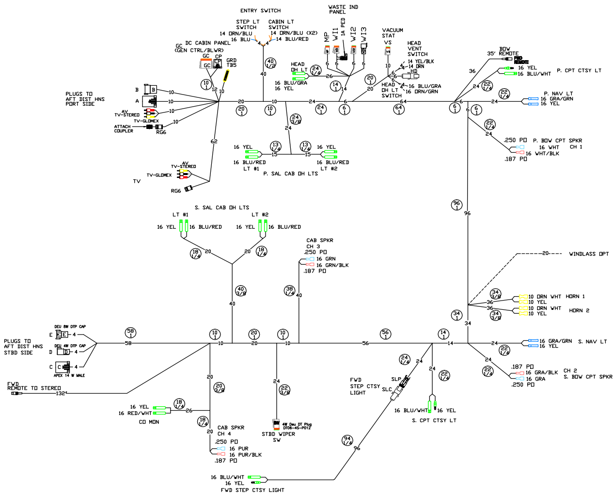
FORWARD DC DISTRIBUTION HARNESS
