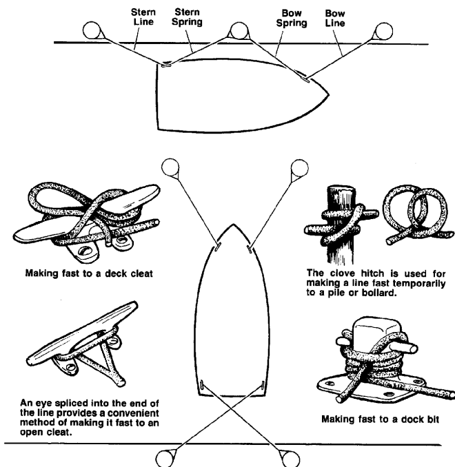
Figure 5.6 Mooring Lines
