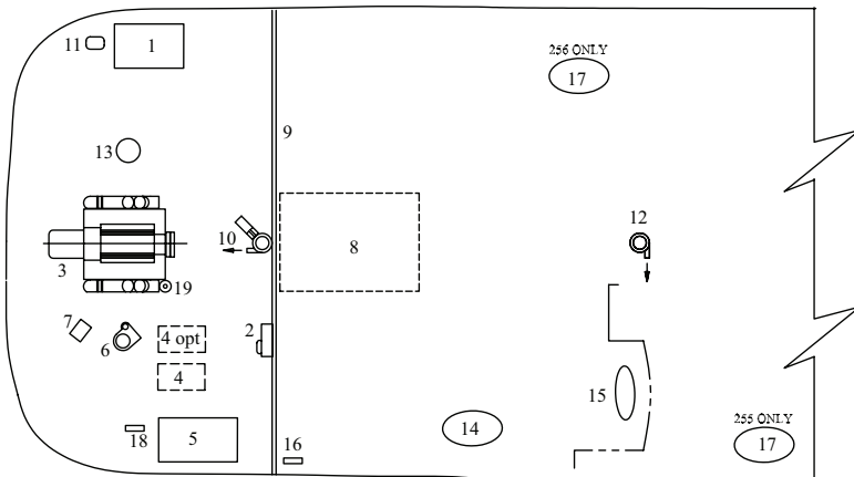
TYPICAL 256, 255 SSI ENGINE COMPARTMENT LAYOUT
