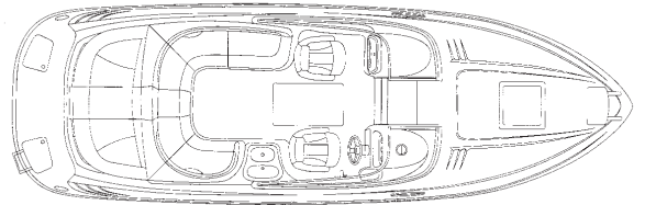
255 SSI DECK PLAN
