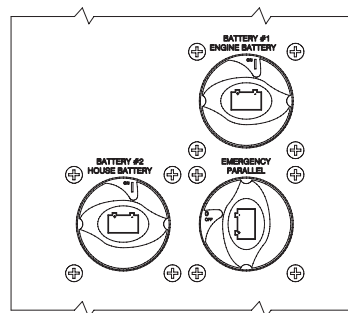
Figure 3.1 275 SSI Battery Panel
