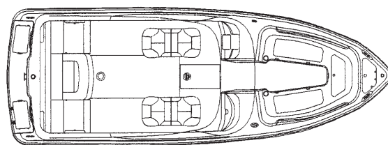
204 SSI STANDARD SEATING DECK PLAN (SPORT SEATING NOT SHOWN)
