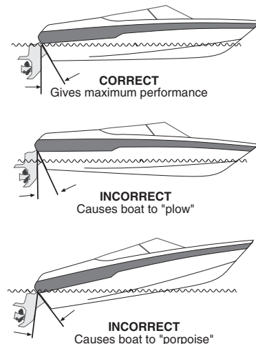
Figure 5.3 Trimming the Drive Angle
