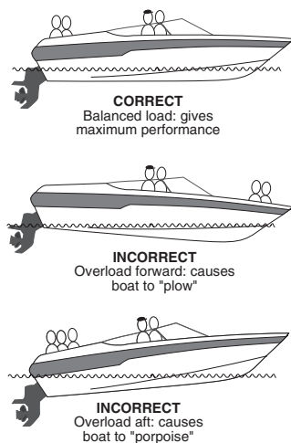
Figure 5.1 Boat Loading
