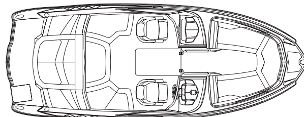
216 SSI WIDE TECH DECK PLAN
