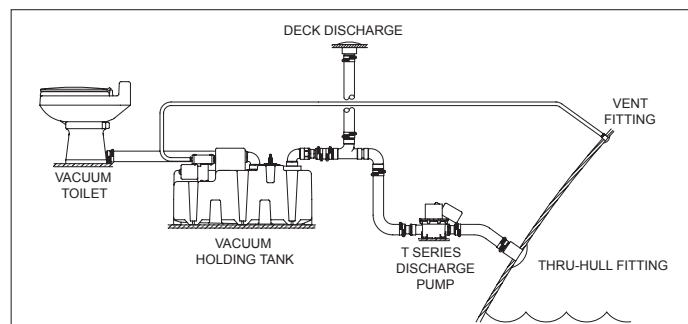
Figure 3.3 VacuFlush® Head
