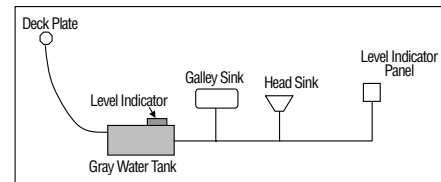
Figure 3.4 Gray water System
