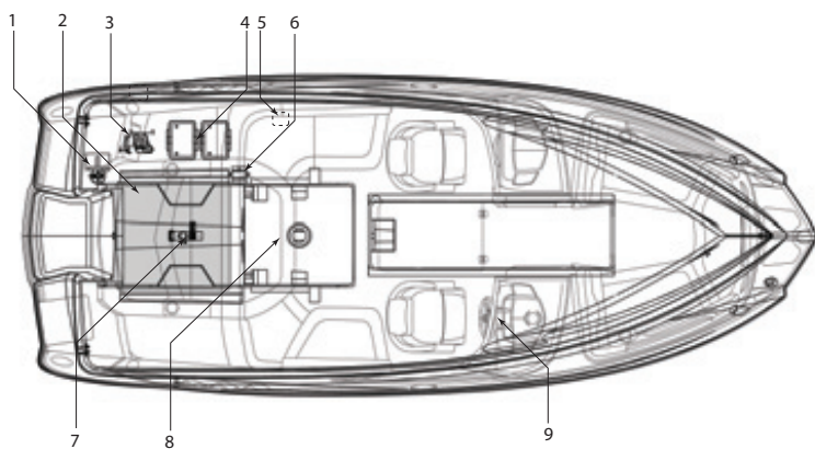
TYPICAL SSI ENGINE COMPARTMENT LAYOUT
