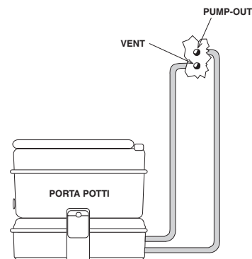
Figure 3.2 Pumpout Porta-Potti
