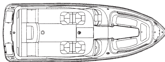
210 SSI STANDARD SEATING DECK PLAN
