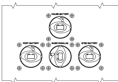
Figure 3.2 280, 290, 310, 330, 350 Battery Panel
