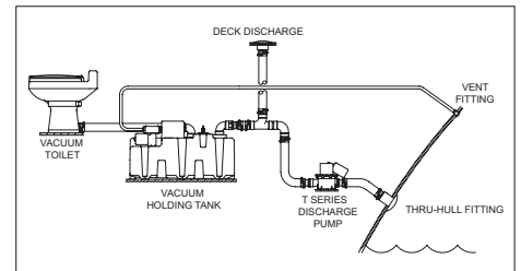
Figure 3.4 VacuFlush® System
