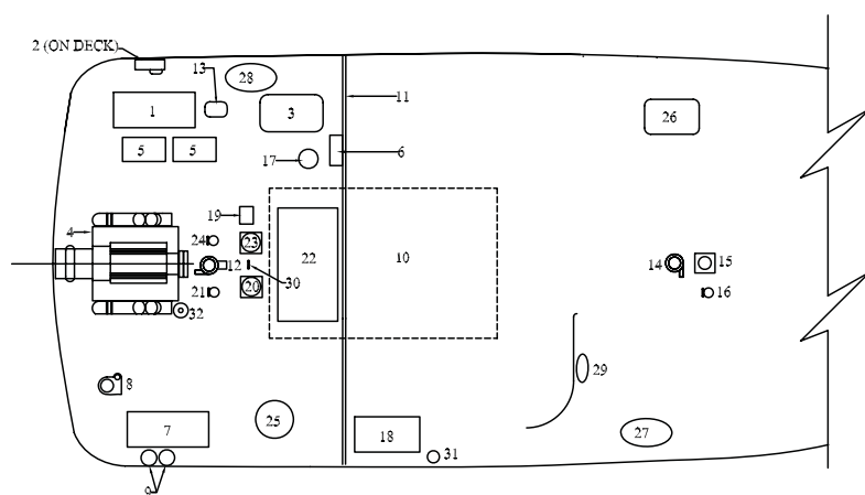
TYPICAL SIGNATURE 270 ENGINE COMPARTMENT LAYOUT
