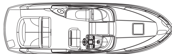
SIGNATURE 250 OPTIONAL DECK PLAN
