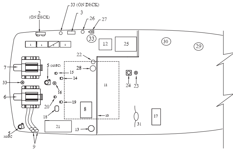
SIGNATURE 310 ENGINE COMPARTMENT
