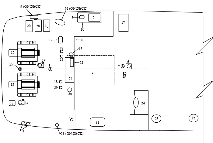
TYPICAL SIGNATURE 280 ENGINE COMPARTMENT
