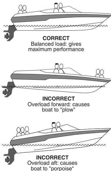
Figure 5.1 Boat Loading
