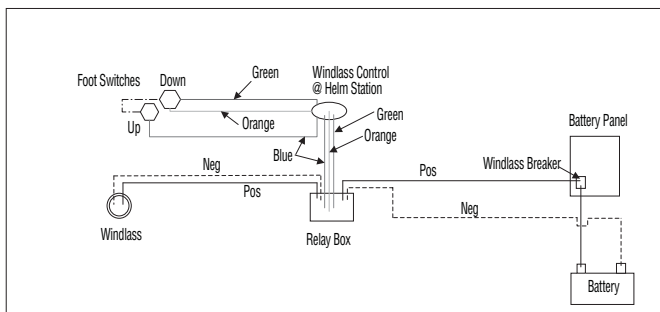
Figure 4.1 Windlass Schematic
