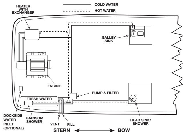
Figure 3.3 Potable Water System
