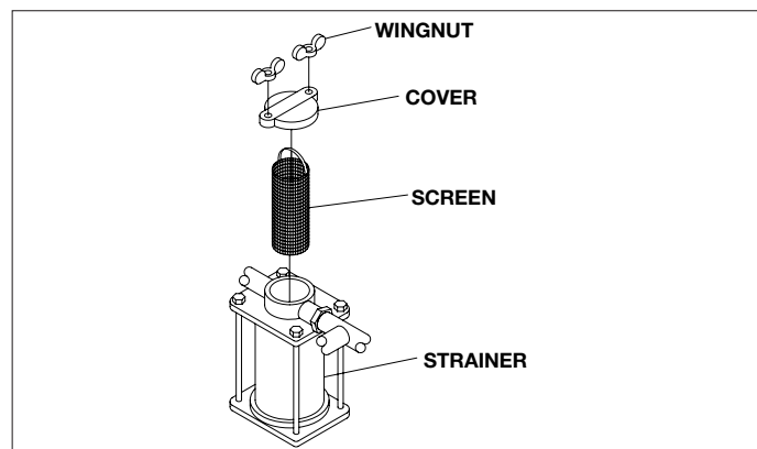
Figure 3.6 Sea Strainer
