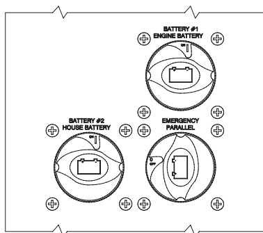
Figure 3.1 270, 250 Battery Panel
