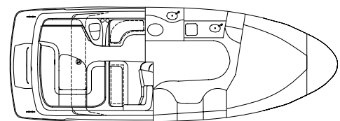
SIGNATURE 280 DECK PLAN
