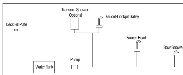
Pressure Water System
