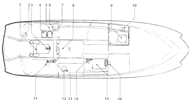
TYPICAL SUNESTA ENGINE COMPARTMENT LAYOUT
