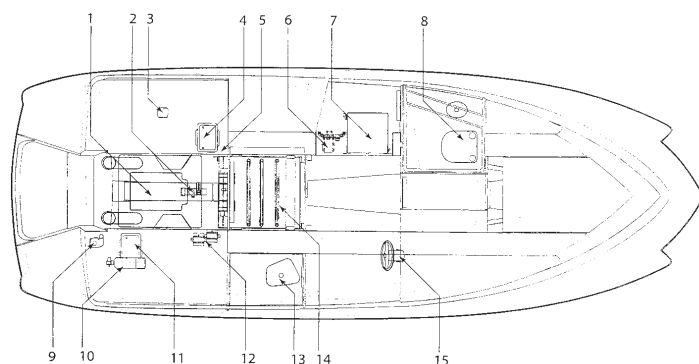
TYPICAL 224 & 244 SUNESEA SYSTEM LAYOUT
