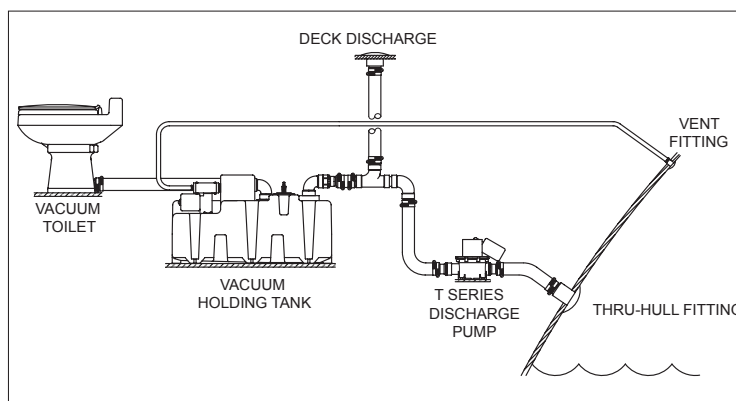
Figure 3.2 VacuFlush® Head
