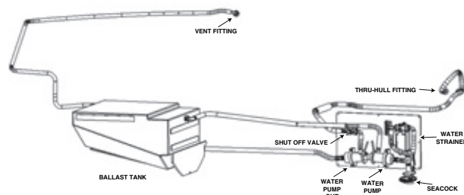
Figure 4.1 Ballast System
