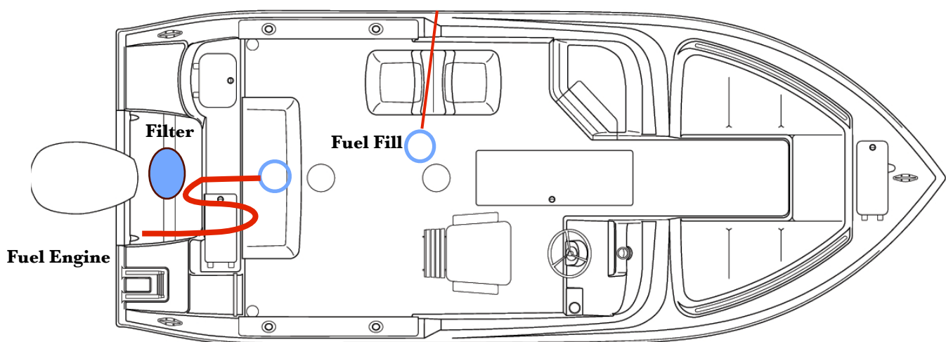
FUEL SYSTEM DIAGRAM
