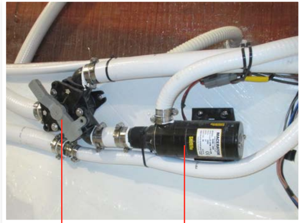
Y-Valve
