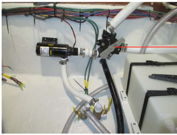
Y-Valve
