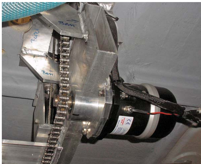
Autopilot drive TS250 mounted in a Hanse 630
