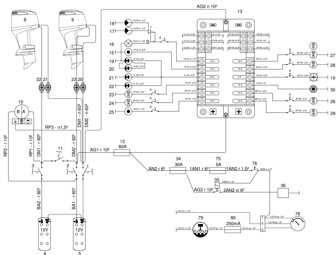
ELECTRICITY - SCHEMA
