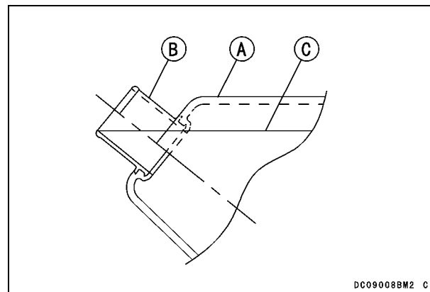
A. Fuel Tank B. Filler Neck C. Top Level
