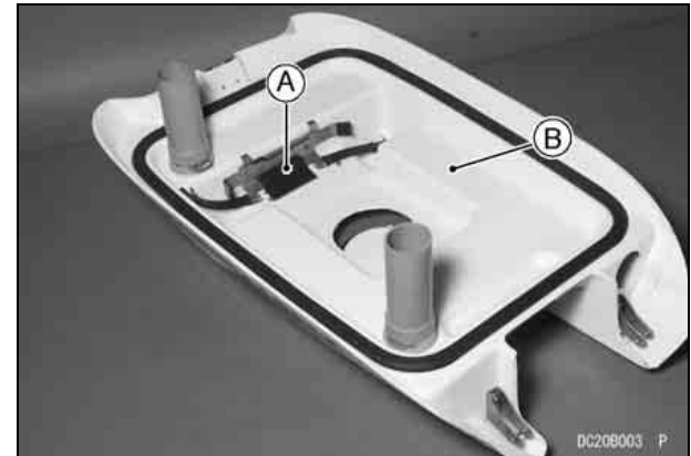
A. Fire Extinguisher Holder B. Engine Cover
