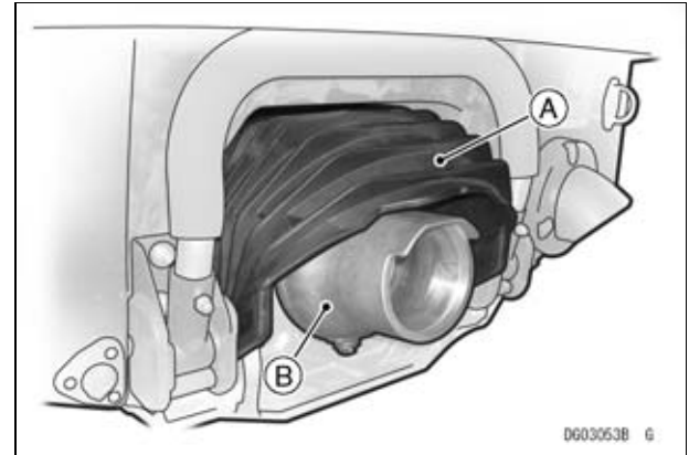
A. Reverse Bucket B. Steering Nozzle
