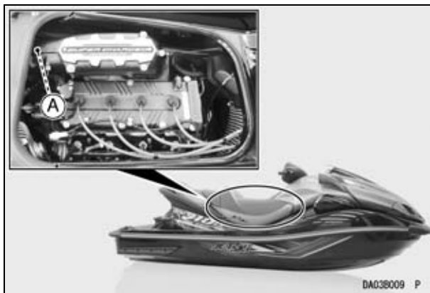
A. Exhaust Filter
