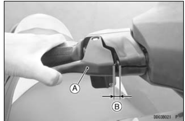
A. Throttle Lever B. about 2 mm (0.08 in.)
