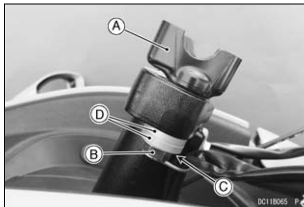
A. Handlebar Holder B. Handlebar Holder Nut C. Washer D. Collars
