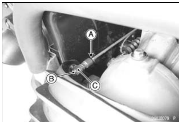
A. Locknut B. Ball Joint C. Sleeve
