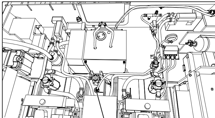
AIR CONDITIONER SEAWATER INTAKE SEACOCK
