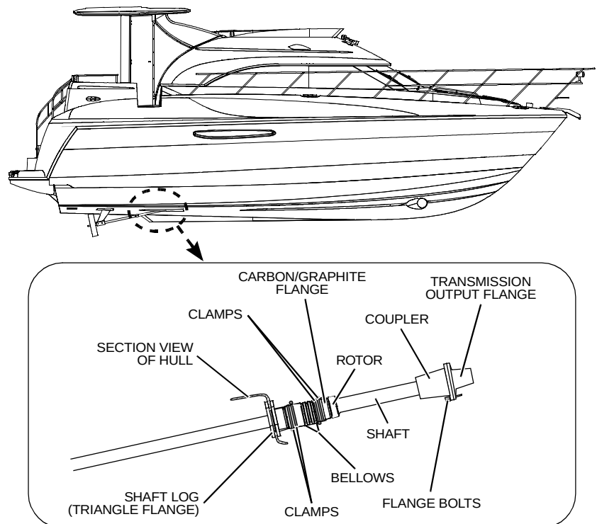
TRANSMISSION-TO-PROP SHAFT COMPONENTS (TYPICAL)
