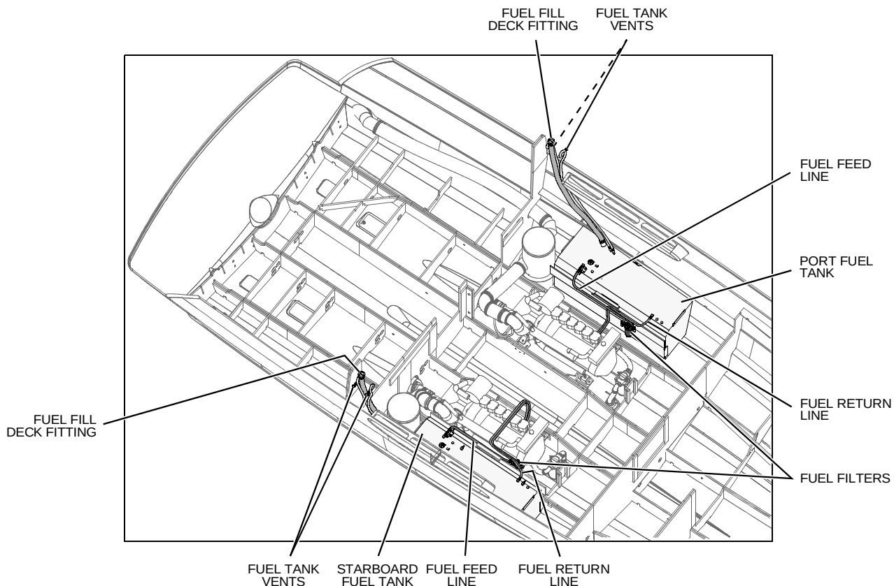
DIESEL FUEL LINE ROUTING (IF EQUIPPED)
