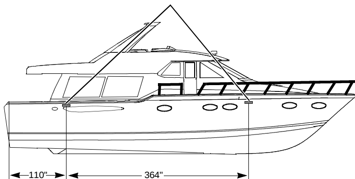
LIFTING SLING LABELS (TYPICAL PORT & STARBOARD)
