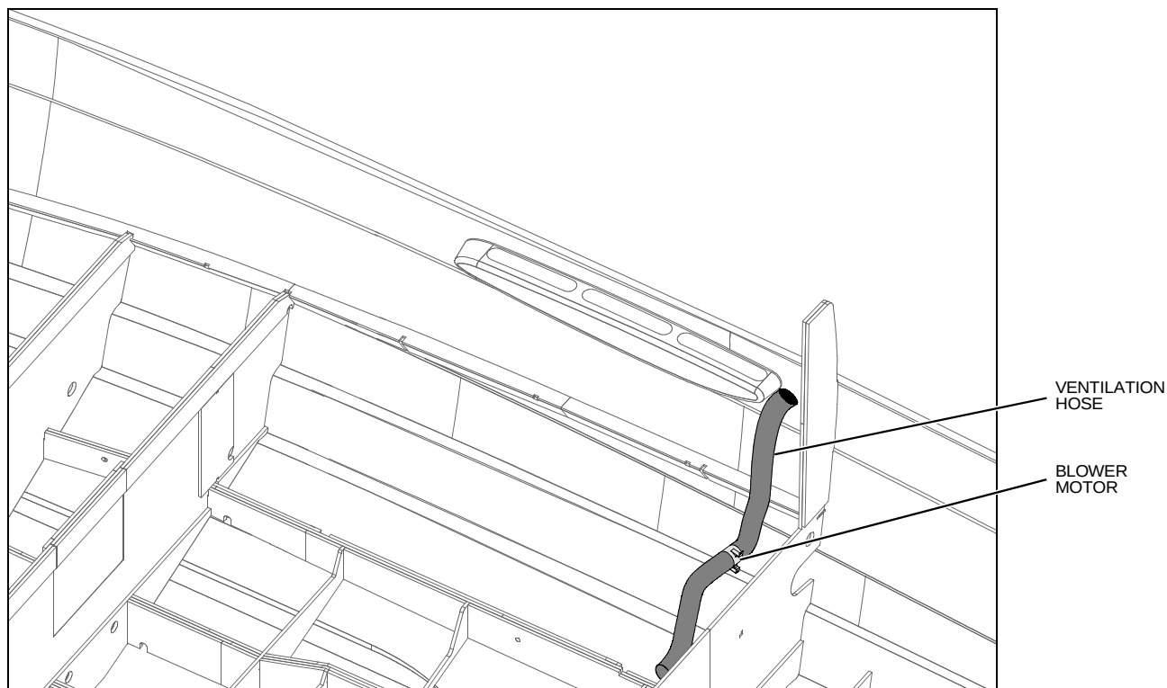
BILGE BLOWER SYSTEM ROUTING (TYPICAL)
