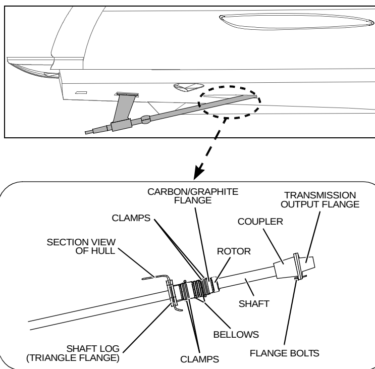
TRANSMISSION-TO-PROP SHAFT COMPONENTS (TYPICAL)
