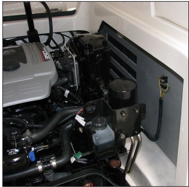
Port Storage Compartment Vents Located in Engine Compartment
