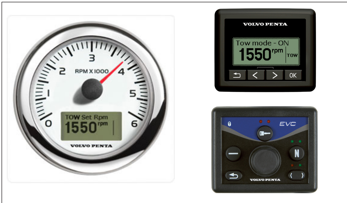
Volvo Aquamatic Tow Control Tachometer, Tow Control Panel and EVC Panel
