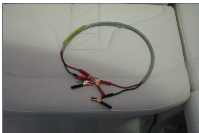
Emergency Engine Hatch Jumper Harness
