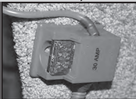
Fuse Panel - Battery Connection
