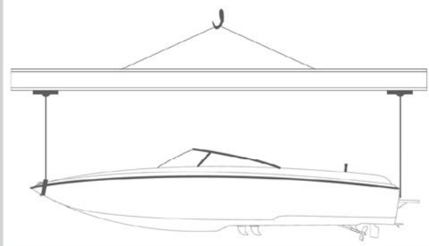
CORRECT HOISTING
