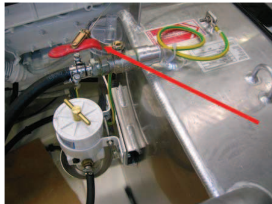
VALVE DIESEL ENGINE REF. 1, 2
