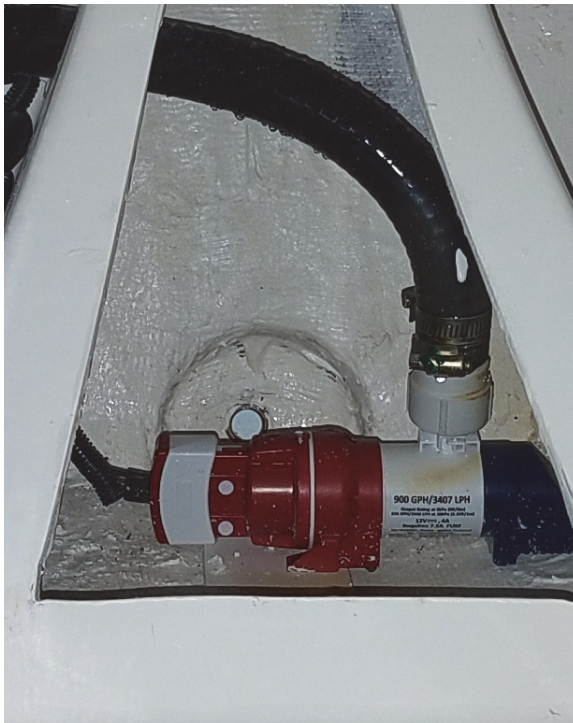
DC 235 Bilge Pump
