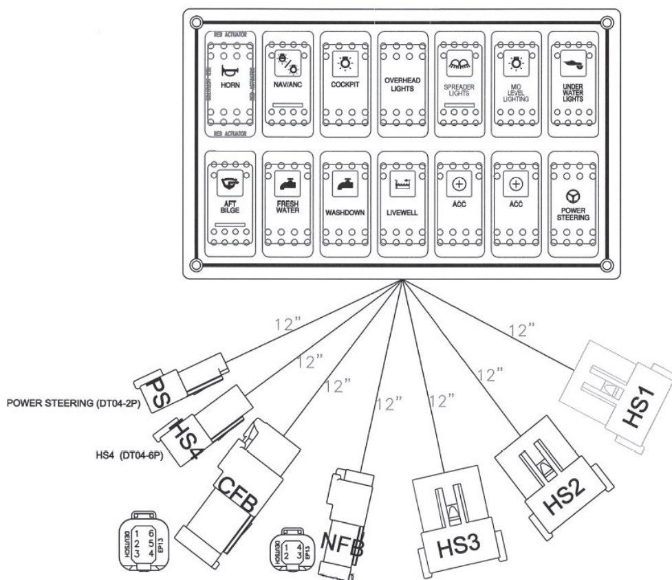
Helm Panel DC235
