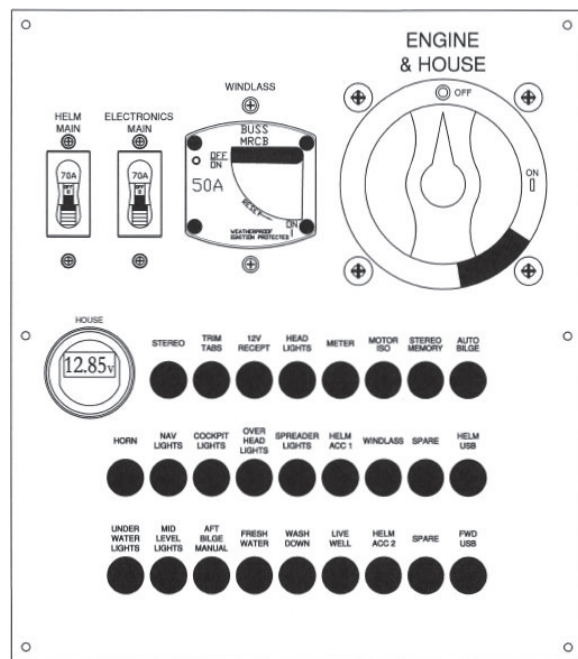
Main Distribution Panel DC235
