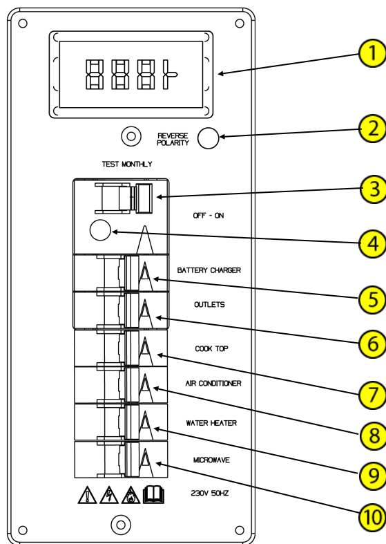
AC Panel
