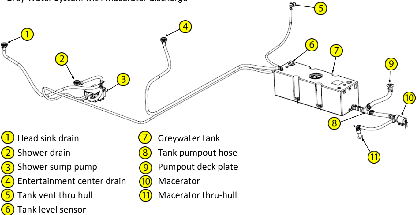
Grey Water System with Macerator discharge
