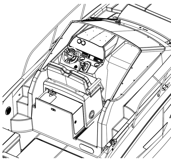
Helm Seat — Forward Position
