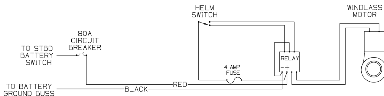
Bow Windlass Schematic
