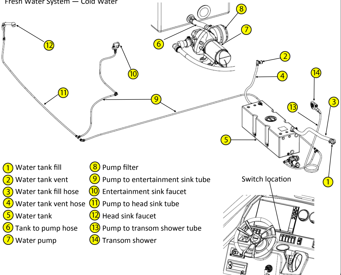
Fresh Water System — Cold Water
