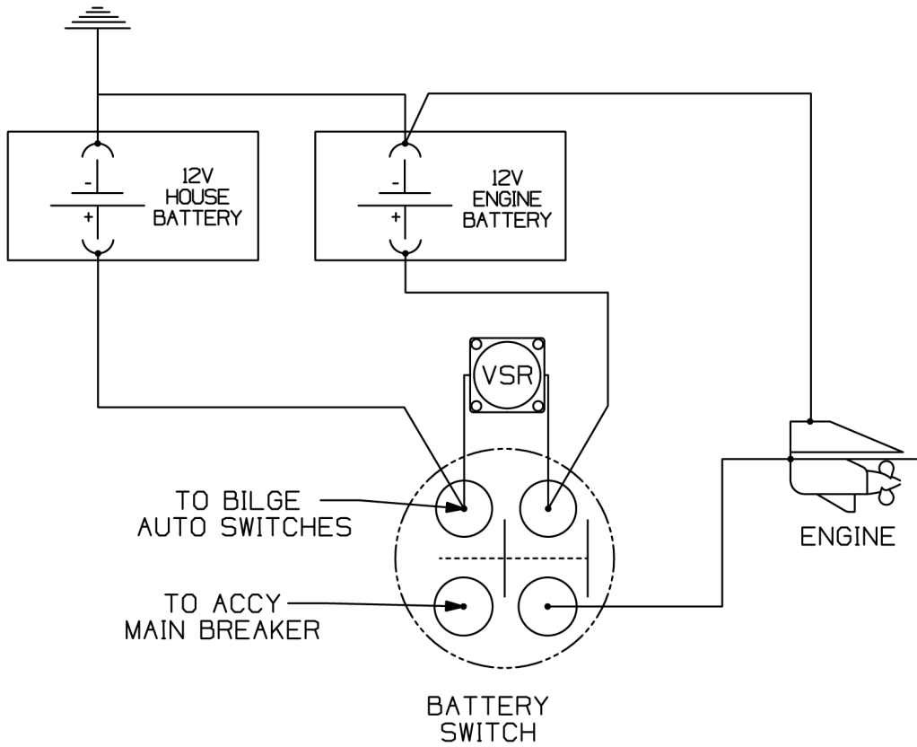
Single Engine Battery Schematic
