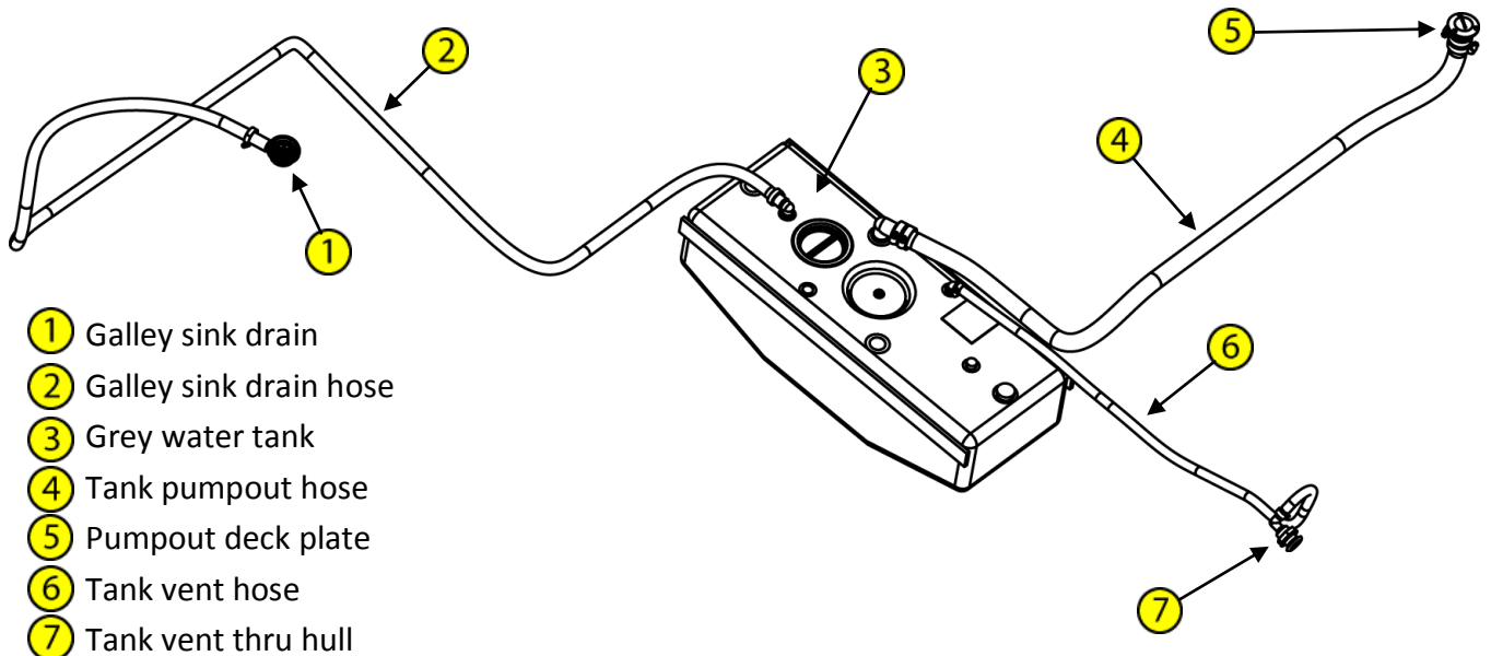
Grey Water System
