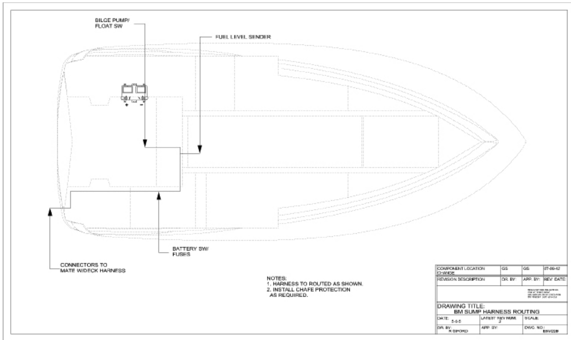
Sump Harness Routing
