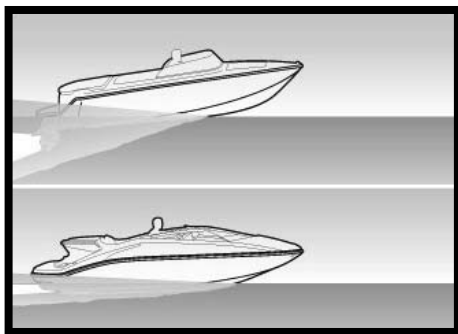
Boat While Planing
