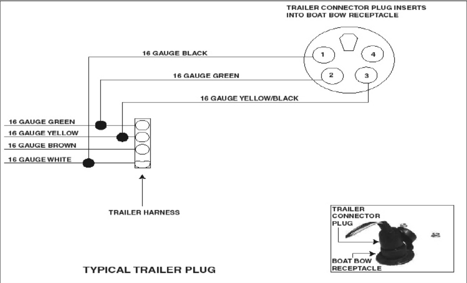
Trailer Harness Plug
