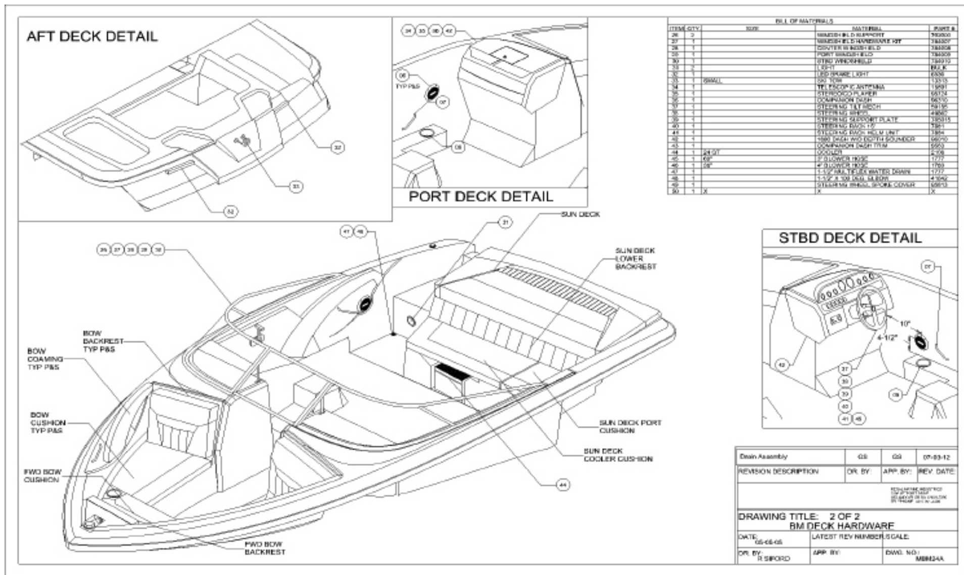
Deck Hardware 2 of 2
