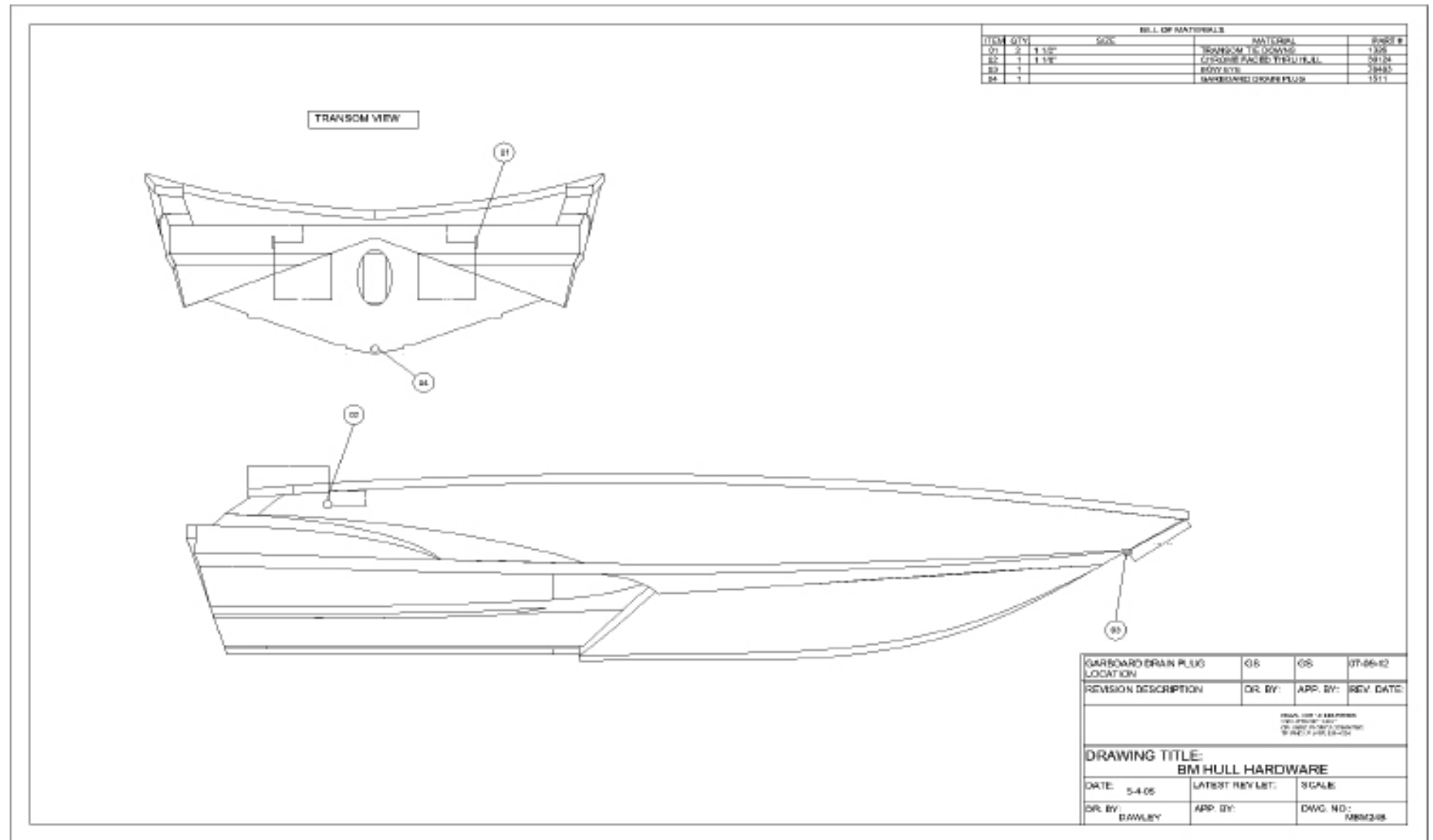
Hull Hardware
