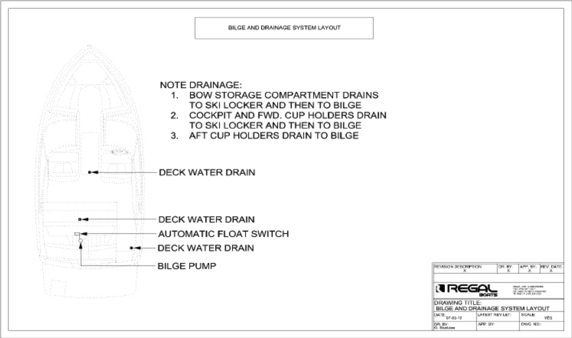
Bilge And Drainage Diagram
