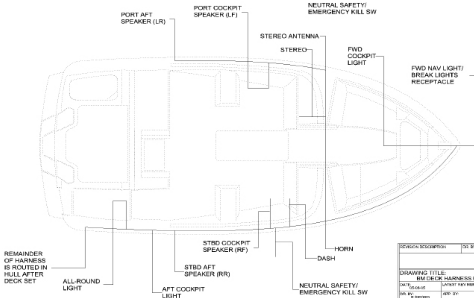
Deck Harness Routing
