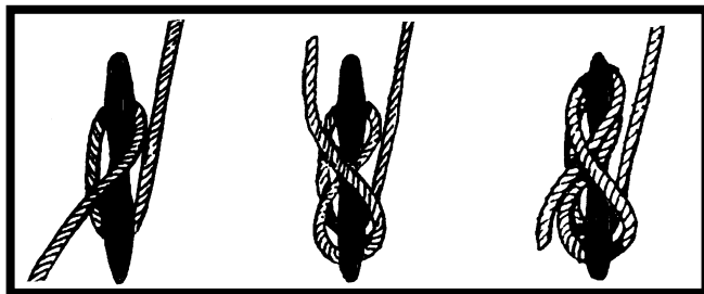
Figure Eight Knot Tie To Cleat
