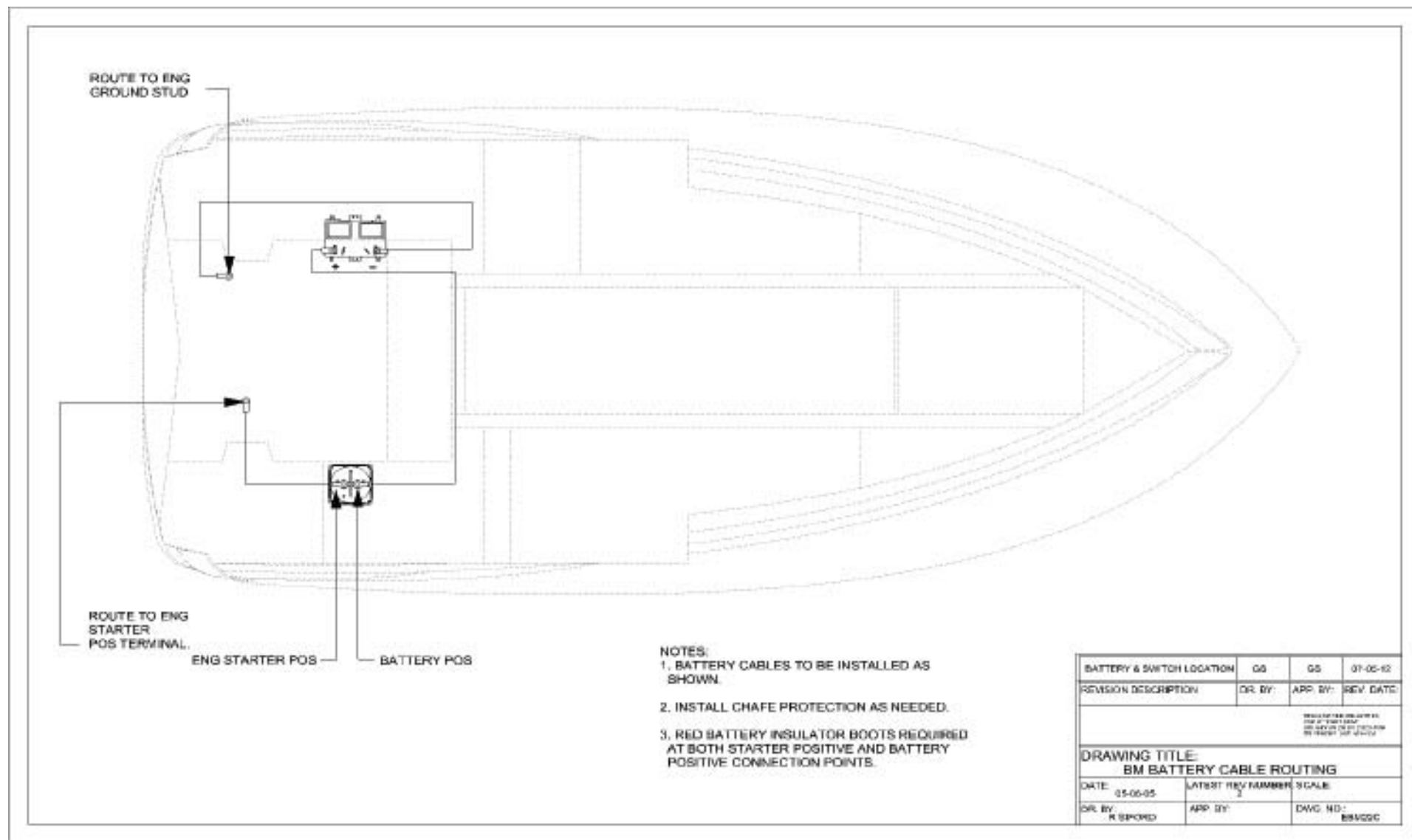
Battery Cable Routing
