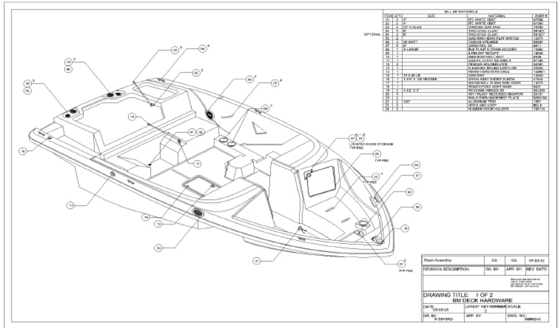
Deck Hardware 1 of 2
