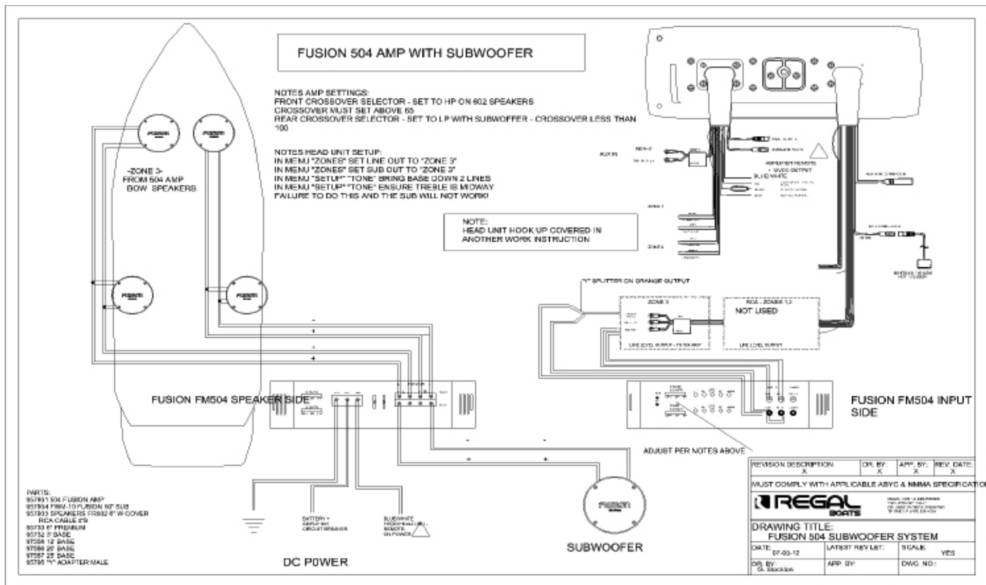
Fusion Stereo Optional Performance Package Connection
