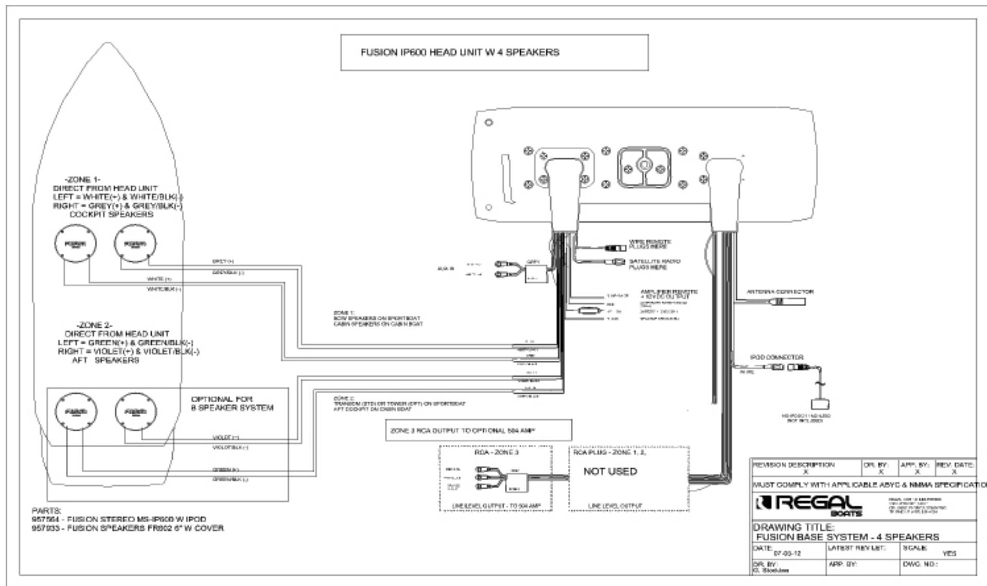
Fusion Stereo Connection
