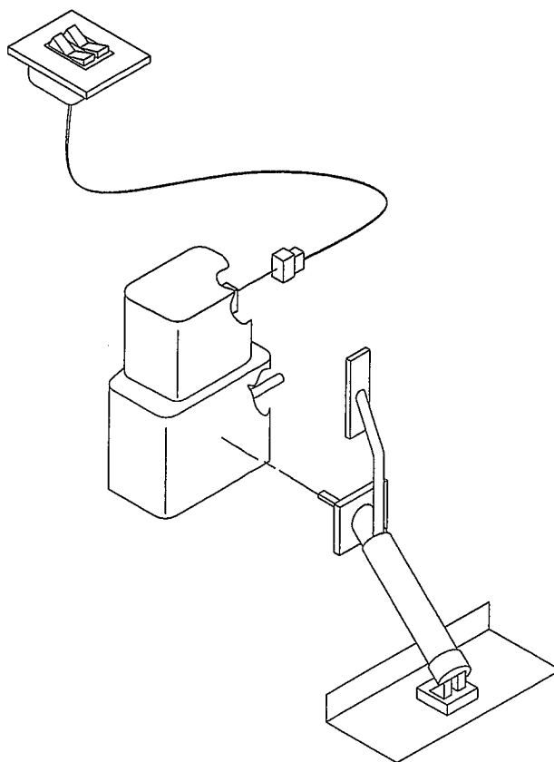
FIGURE 5.7 TRIM TAB, RESERVOIR AND SWITCH
