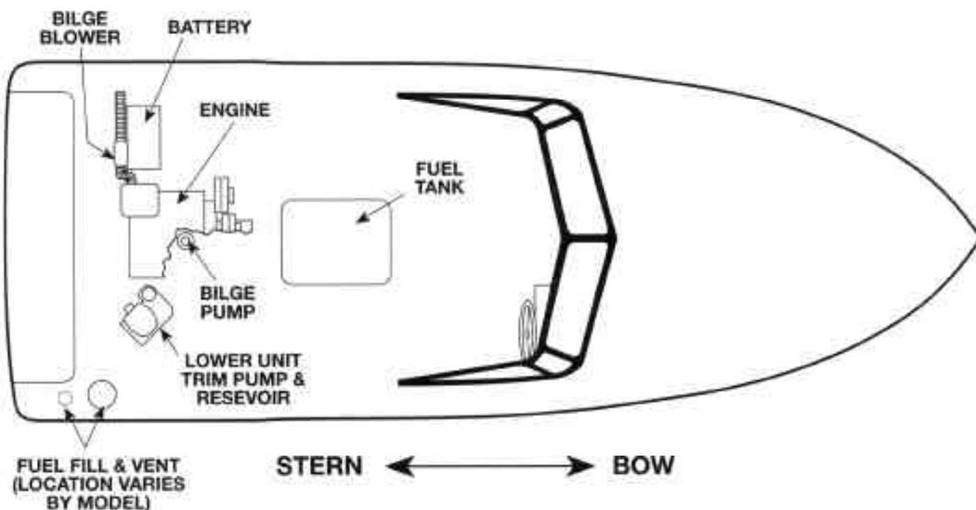
FIGURE 3.1 EQUIPMENT LOCATOR
