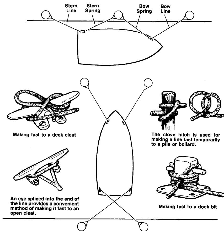
Figure 5.6 Mooring Lines
