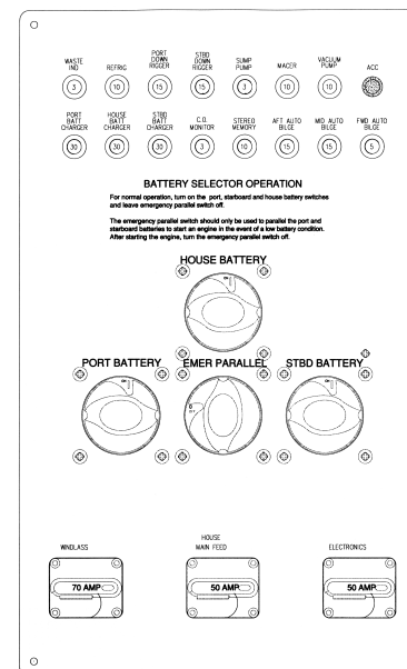
Figure 3.1 Four Selector Switches with Three Batteries and Twin Engines
