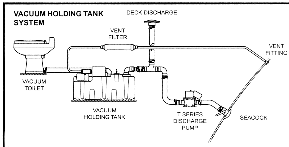
Figure 3.5 VacuFlush® Head
