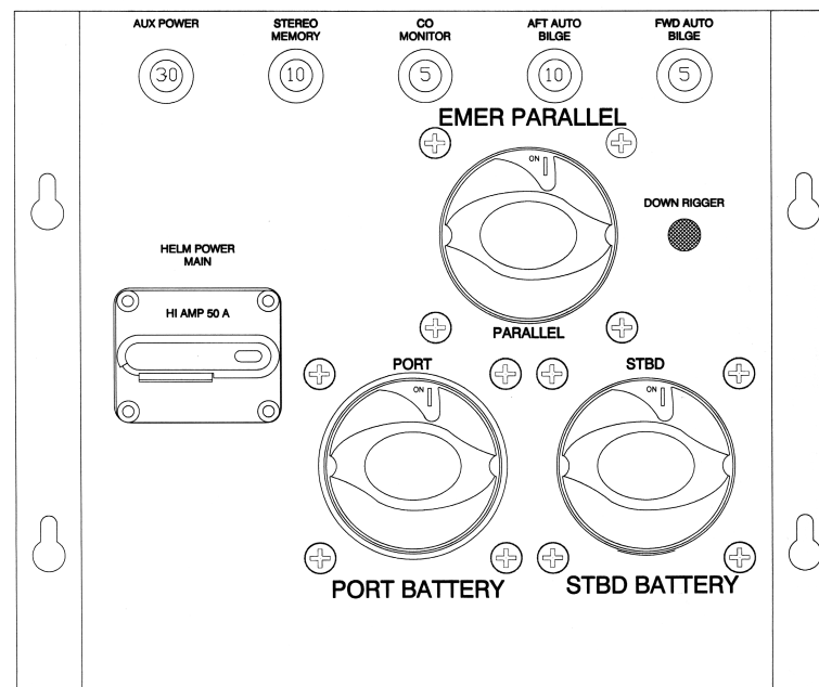
Figure 3.3 Three Selector Switches with Two Batteries and Single Engine
