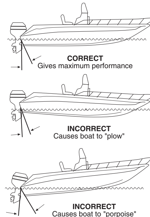
Figure 5.3 Trimming the Drive Angle
