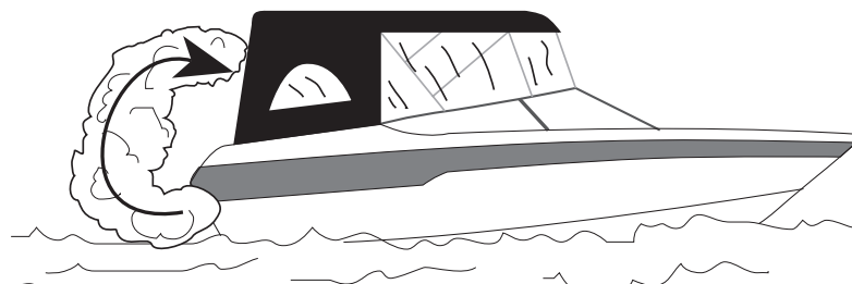
Figure 2.3 Exhaust Accumulation While Canvas is in Place
