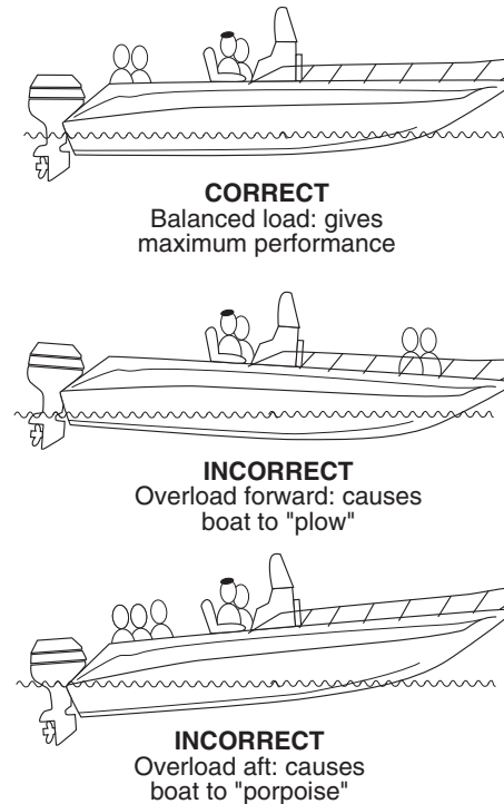
Figure 5.1 Boat Loading
