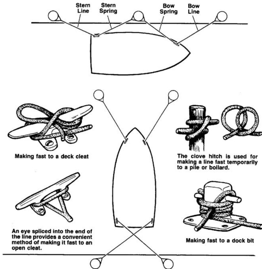
Figure 5.6: Mooring Lines
