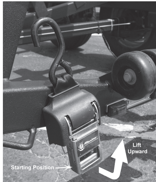
Figure F14: Rear Tie Down Strap - Tightening
