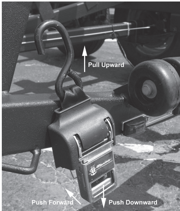
Figure F13: Rear Tie Down Strap - Release
