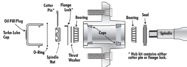
Figure F20: Axle Components
