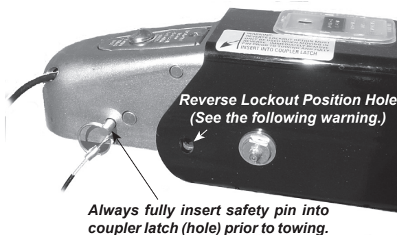
Figure F17: Reverse Manual Brake Lockout
