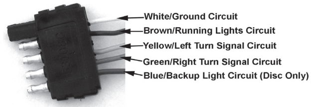
Figure F7: 5-Wire Plug Harness
