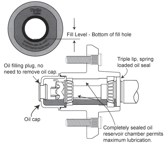
Figure F19: Turbo Lube Oil Fill Diagram
