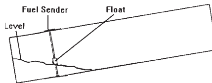
Figure B29: Trim Angle Effect with Low Fuel
