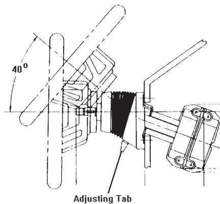
Figure B4: Tilt Steering
