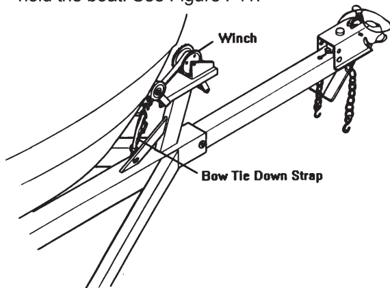
Figure F11: Bow Tie Down Strap
