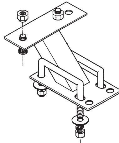
Figure F9: Spare Tire Carrier
