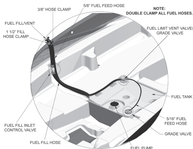
Figure B24: Pressurized Fuel System
