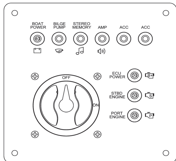
Figure B11: Battery Switch Panel
