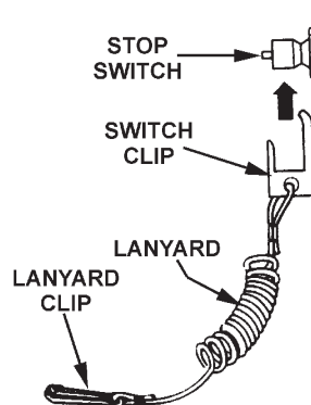
Figure B3: Emergency Engine Shut Off Switch
