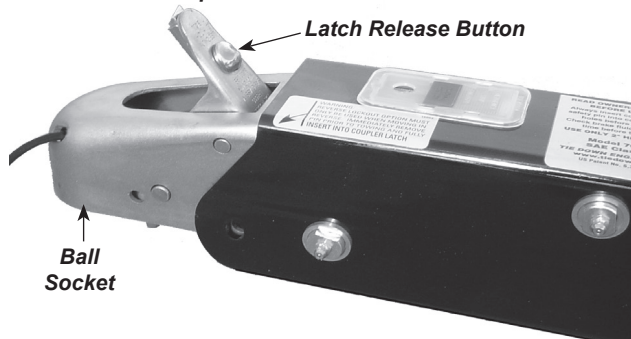
Figure F5: Brake Actuator & Coupling Assembly - Open
