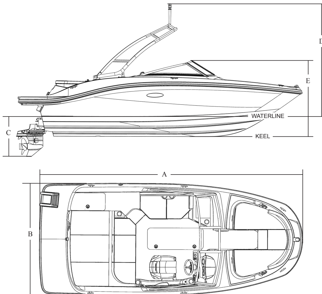
BOAT DIMENSIONS AND CLEARANCES (FIG. 8.1)
