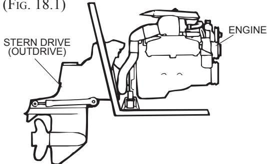
STERN DRIVE (INBOARD-OUTBOARD) ENGINE (FIG. 18.1)
