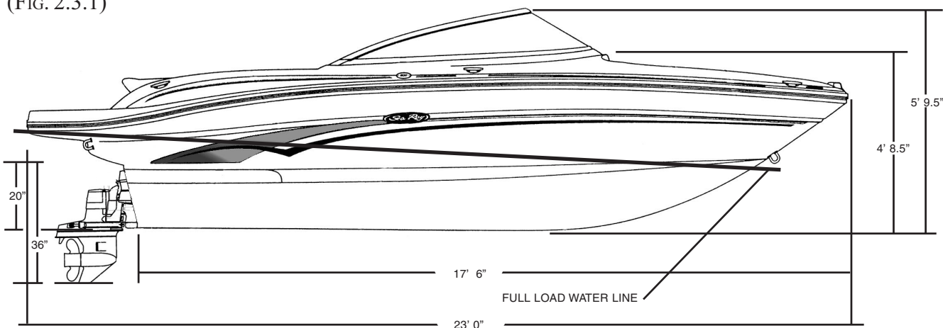
BOAT DIMENSIONS AND CLEARANCES (FIG. 2.3.1)
