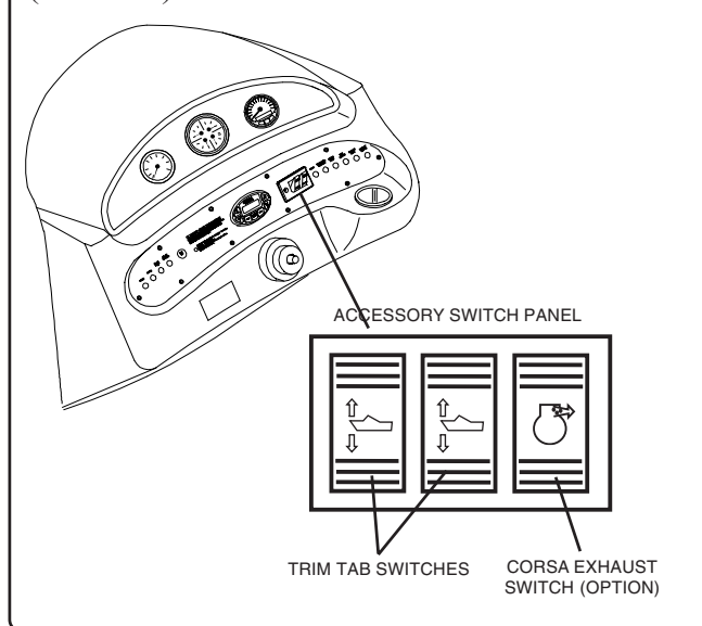
CORSA™ EXHAUST SYSTEM SWITCH (FIG.7.1.1)
