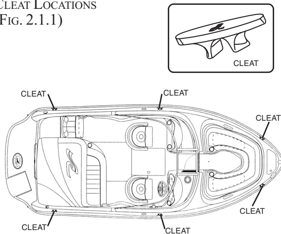
BOW AND STERN EYE LOCATIONS (FIG. 2.1.2)
