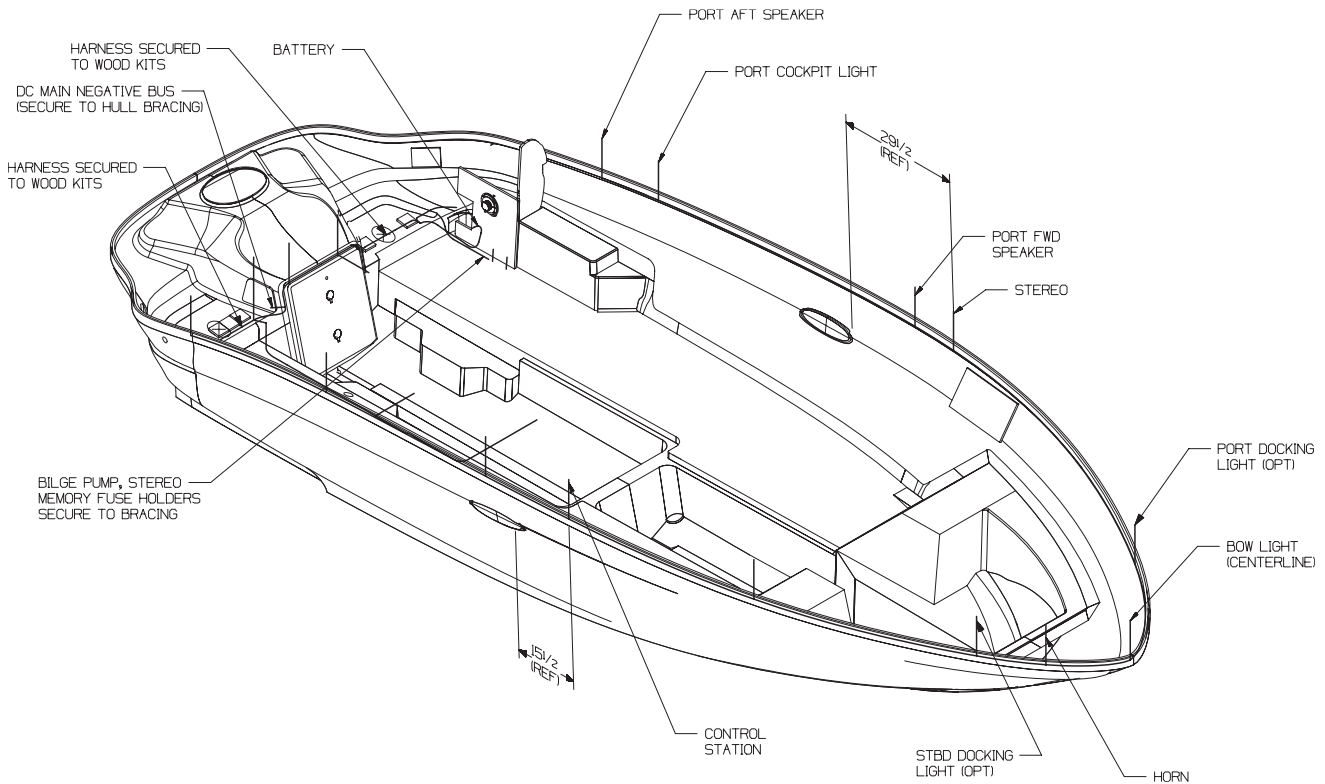
WIRE HARNESS (FIG. 6.8.1)
