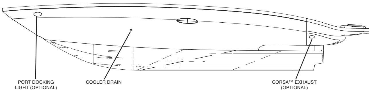
PORT THROUGH-HULL CUTOUTS (FIG. 2.6.2)
