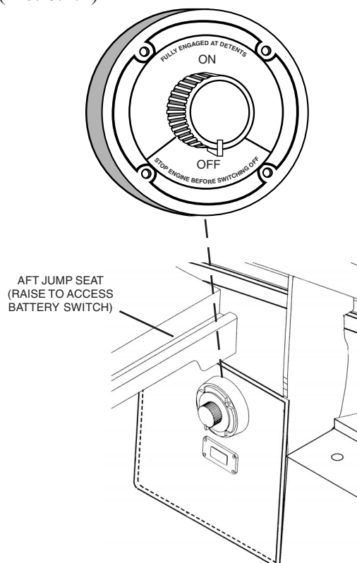
BATTERY SWITCH (FIG. 6.4.1)
