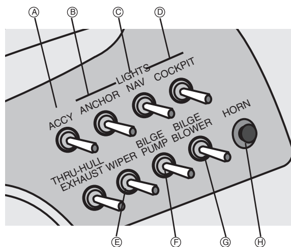
ELECTRONIC SWITCH PAD (FIG. 6.5.4)
