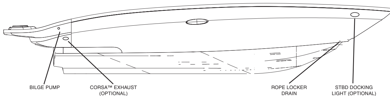
STARBOARD THROUGH-HULL CUTOUTS (FIG. 2.6.1)
