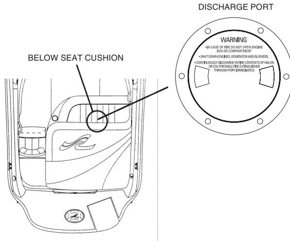
FIRE EXTINGUISHER DISCHARGE PORT (FIG. 7.6.1)
