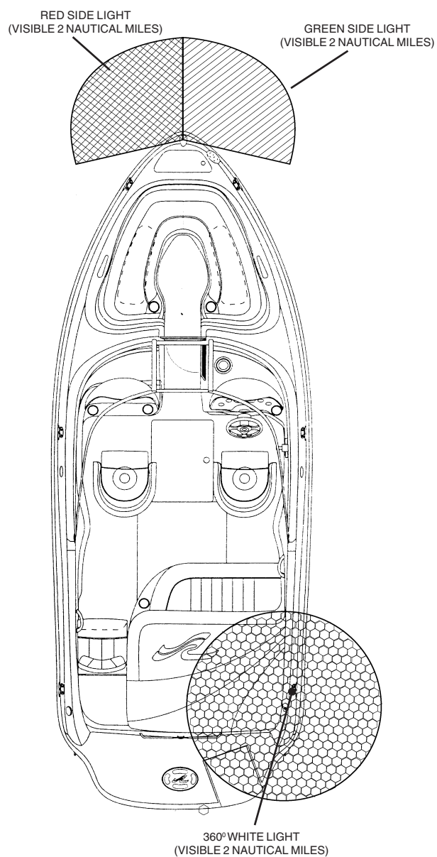
NAVIGATION AND ANCHOR LIGHTS (FIG. 2.12.1)
