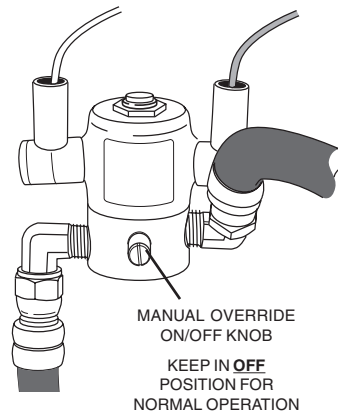
TYPICAL ELECTRIC FUEL VALVE (FIG. 5.1.2)
