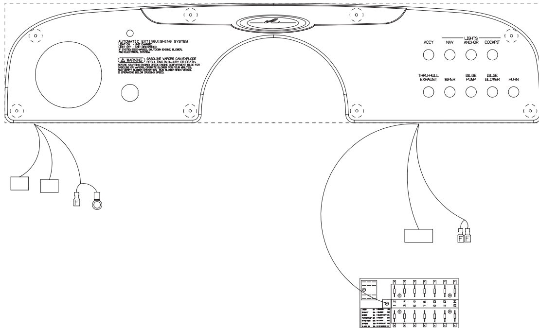
CONTROL STATION SWITCH HARNESS (FIG. 6.9.1)
