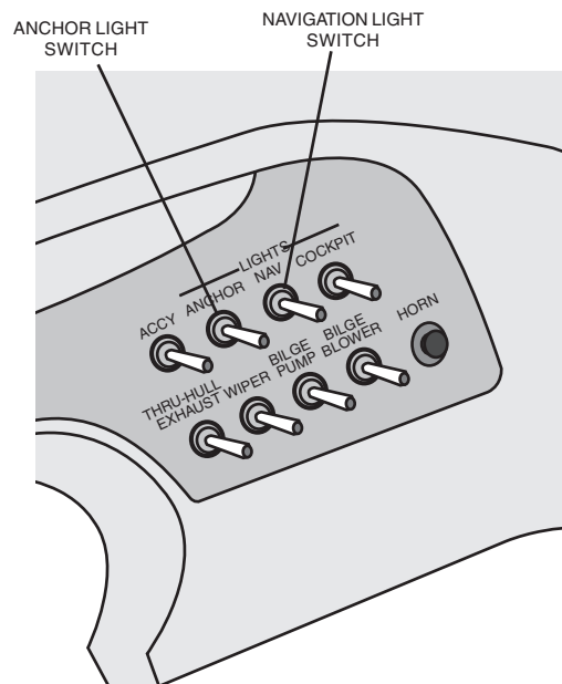
NAVIGATION AND ANCHOR LIGHT SWITCHES (FIG. 2.11.1)
