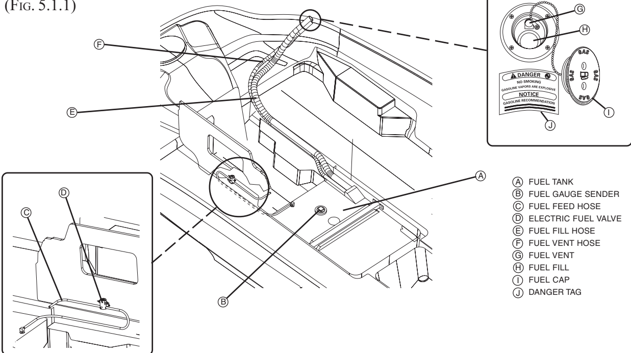
FUEL LINE ROUTING (FIG. 5.1.1)
