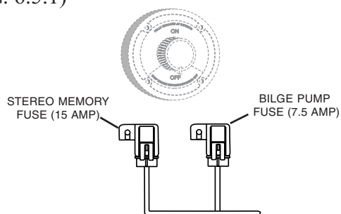
STEREO MEMORY/BILGE PUMP FUSES (FIG. 6.5.1)
