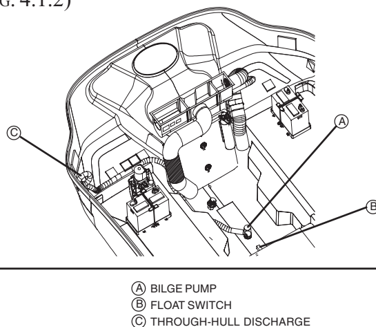
BILGE PUMP AND FLOAT SWITCH (FIG. 4.1.2)
