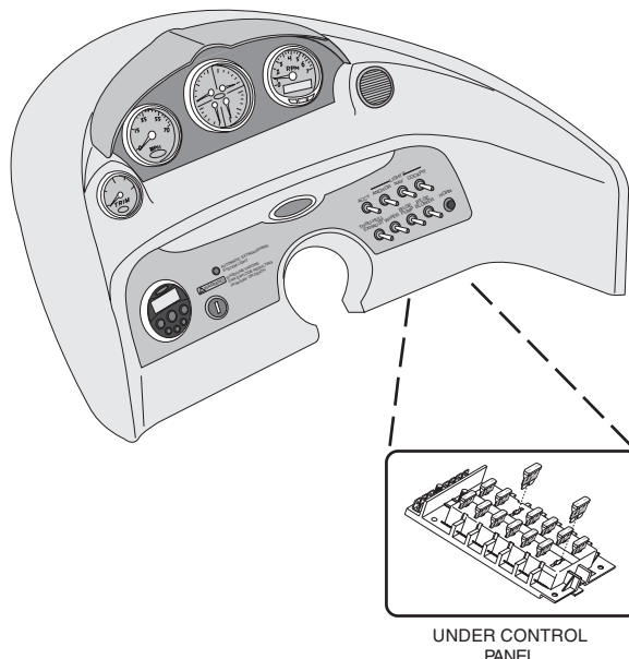
FUSE PANEL LOCATION (FIG. 6.6.1)
