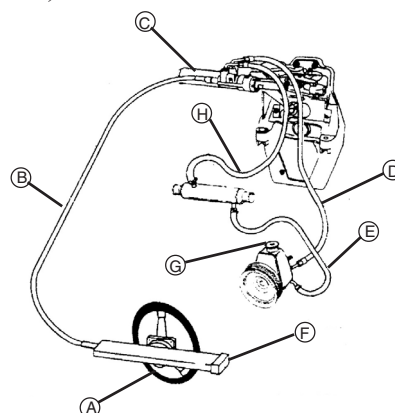
POWER STEERING SYSTEM (FIG. 3.7.4)
