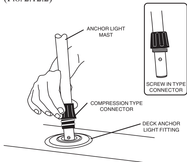
INSERTING THE REMOVABLE STERN ANCHOR LIGHT (FIG. 2.12.2)
