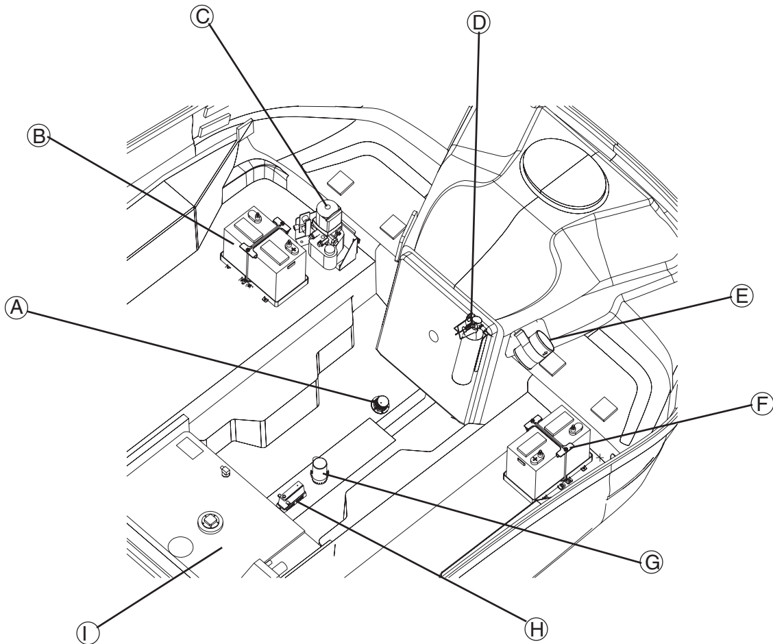
BILGE LAYOUT (OPTIONAL, DUAL BATTERY) (FIG. 4.7.1)
