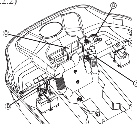
BILGE BLOWER (FIG. 4.2.2)
