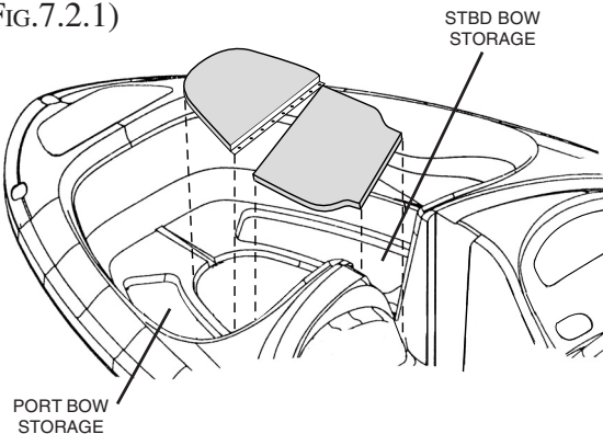
CONVERTABLE BOW SEATING (FIG.7.2.1)
