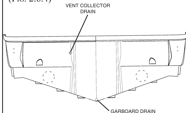
TRANSOM THROUGH-HULL CUTOUTS (FIG. 2.6.4)
