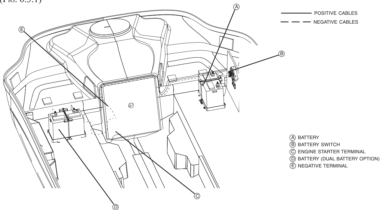
BATTERY CABLE ROUTING (OPTIONAL DUAL BATTERY) (FIG. 6.3.1)
