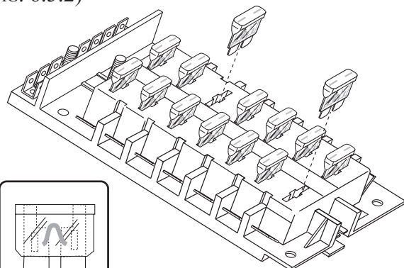
FUSES (FIG. 6.5.2)
