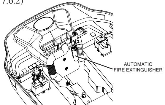
AUTOMATIC FIRE EXTINGUISHER (FIG. 7.6.2)
